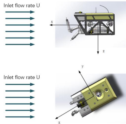
Fig8 flow velocity at the entrance of the solution domain
