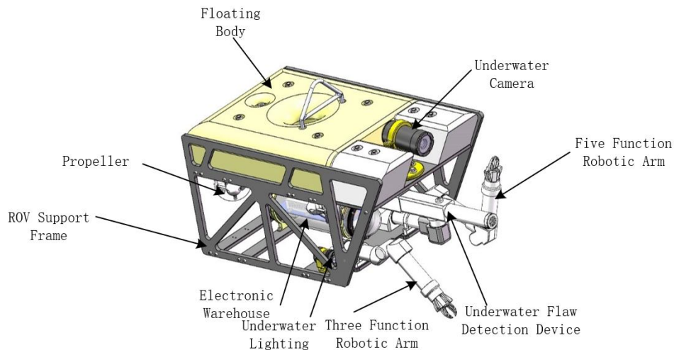
Fig 1 Overall schematic diagram of ROV
