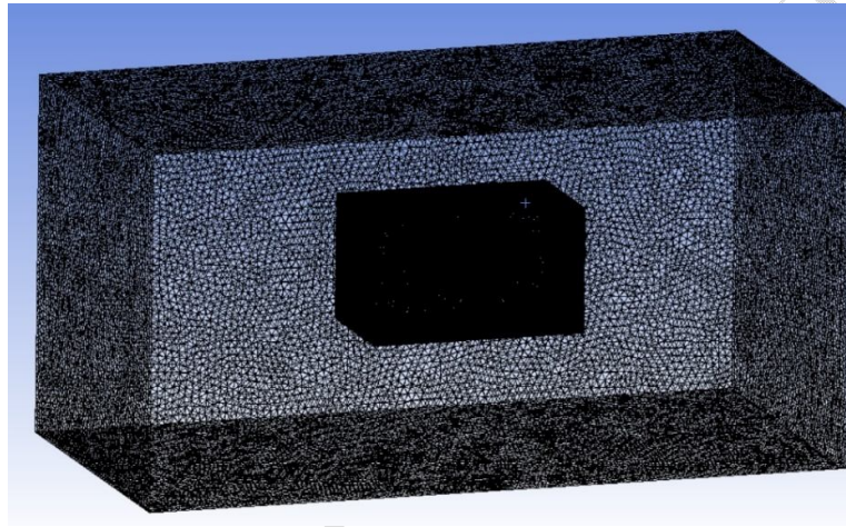
Fig10 Outer basin grid division
