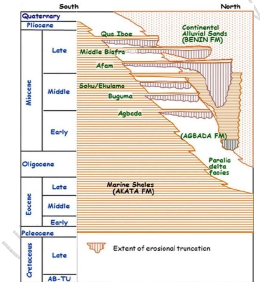
Fig. 2. Regional stratigraphy of the Niger Delta showing different geologic formations (Akata Formation, which is the oldest; Agbada Formation that overlies the Akata and the youngest Benin Formation containing mainly alluvial deposits) (Ozumba, 2013)
