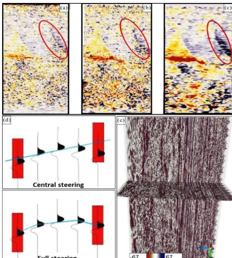
Fig. 3. (a) Full stack steering cube, (b) Detailed steering cube and (c) background steering cube. Notice how the fault on the full stack steering cube was enhanced at the background steered cube. (d) Comparison between central and full steering cube. It appears that the relationship in the full steering cube is better than the centre while the detailed and background steering are better than the full steering cube. (e) Seismic survey base map of the study area displaying seismic inline and cross line. The red box represents the location of the study area.
