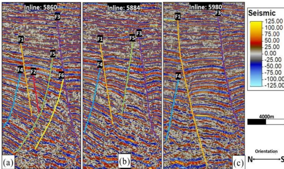
Fig. 5. Interpreted seismic sections of in-lines 5860, 5884, and 5980. Six faults were observed and interpreted on seismic sections A, B and C
