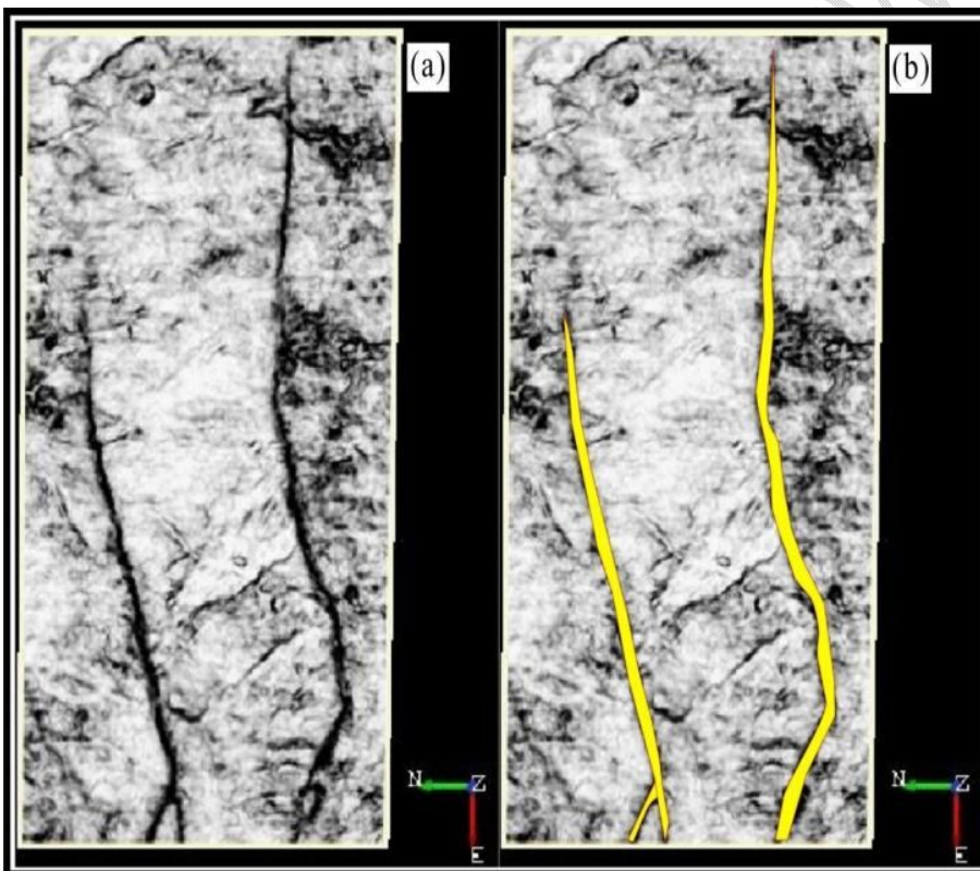
Fig. 6. Extracted similarity attribute maps from inline 5860. (a) shows the uninterpreted map with regions of possible discontinuous reflections. (b) shows the same map with the interpreted faults.
