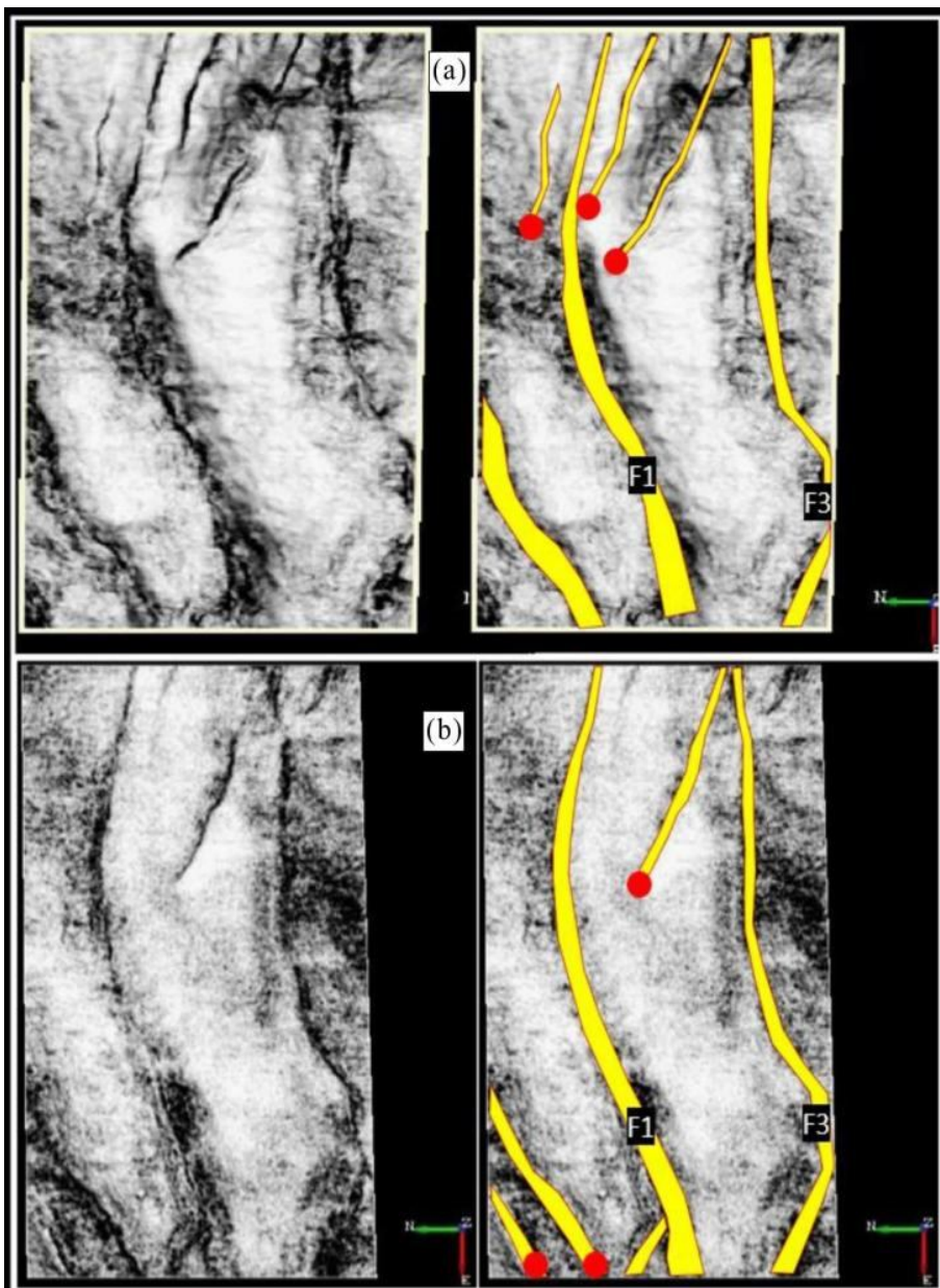
Fig. 7. Extracted similarity attribute maps from inlines 5884 and 5980. On the left of both (a) and (b) are the uninterpreted maps showing regions of possible discontinuous reflections. On the right are the same map with the interpreted faults. F1 and F3 represent fault one and fault three, respectively. The red circles are placed on faults not identified on the seismic sections.
