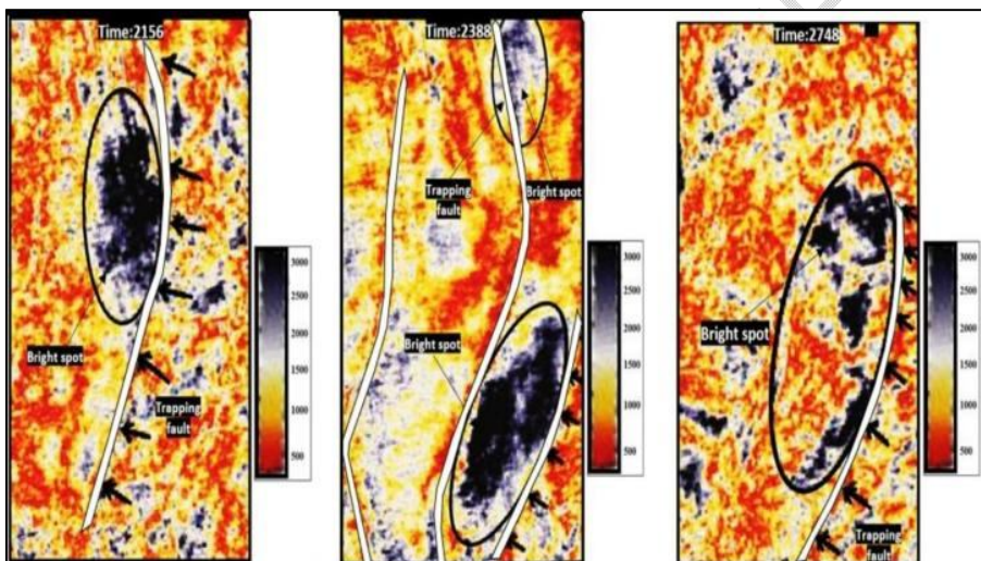
Fig. 8. Time slices showing areas of high amplitude anomalies observed at times 2156, 2388 and 2748, respectively. Using energy attributes, these areas are interpreted as bright spots (potential hydrocarbon areas), and hydrocarbon accumulation was observed to close up on faults.
