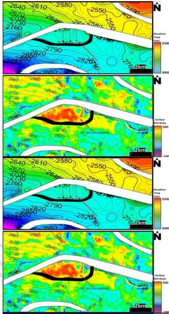
Fig. 10. (a) Interpreted time surface map of a horizon mapped at 2748 showing faults. (b) Contour 2760 is closing on a major fault. The hydrocarbon-bearing region was evident on this attribute map in contour 2760 of the surface map in (a). HC stands for hydrocarbon accumulation
