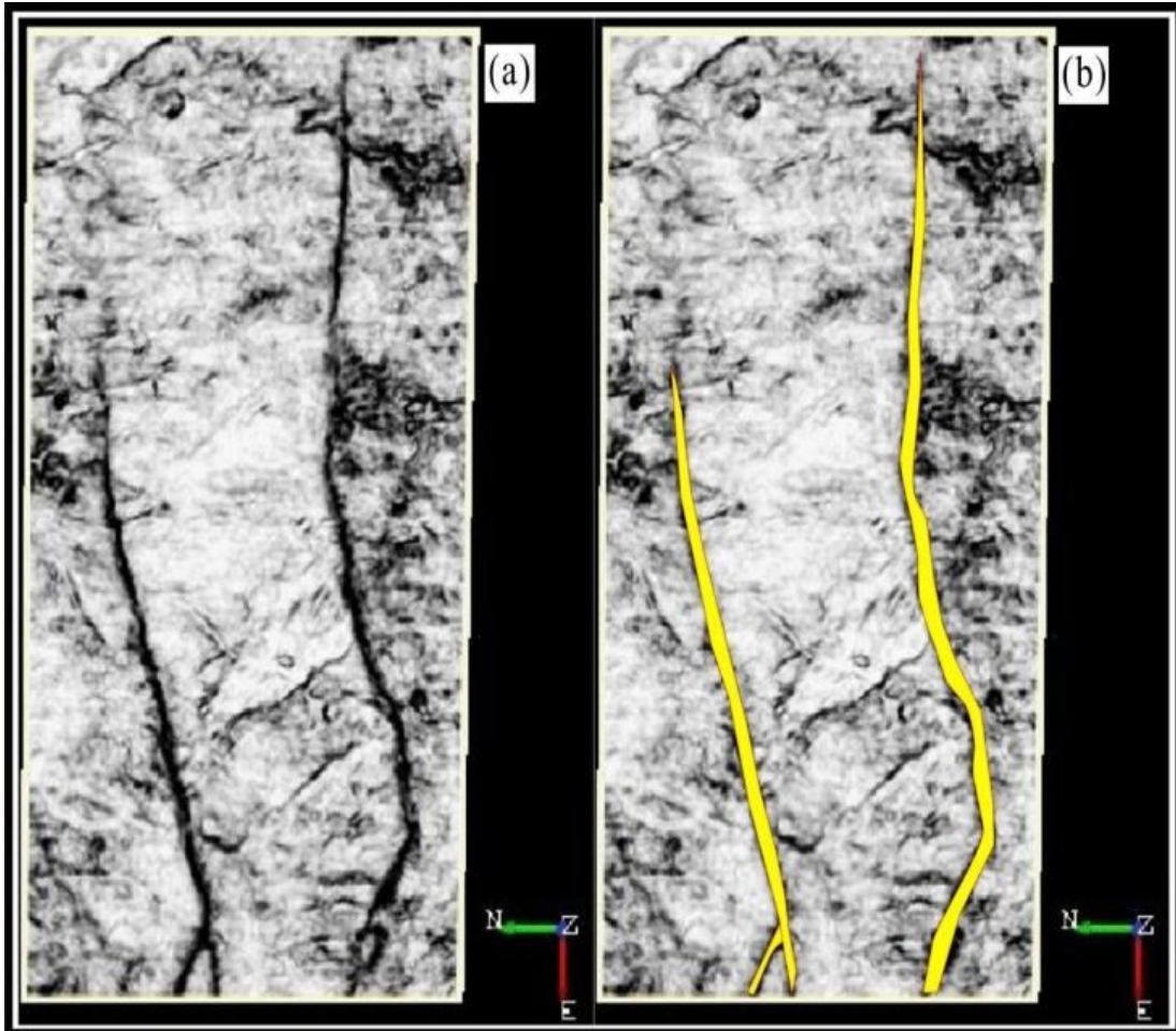
Fig. 6. Extracted similarity attribute maps from inline 5860. (a) shows the uninterpreted map with regions of possible discontinuous reflectionsreflexions . (b) shows the same map withas the interpreted faults.
