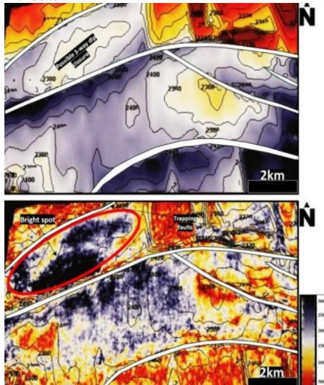
Fig. 9. (a) Time surface map of a horizon mapped at time 2388 with a series of faults dipping in the SW-NE direction. (b) The spectral decomposition map extracted from the OpendTect software. It shows a bright spot region enclosed in a red circle, closing against faults .
