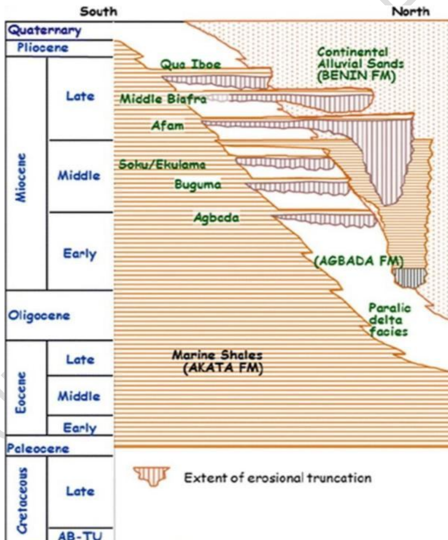
Fig. 2. Regional stratigraphy of the Niger Delta showing different geologic formations (Akata Formation, which is the oldest; Agbada Formation that overlies the overlies Akata and the youngest Benin Formation containing mainly alluvial deposits) (Ozumba, 2013)
