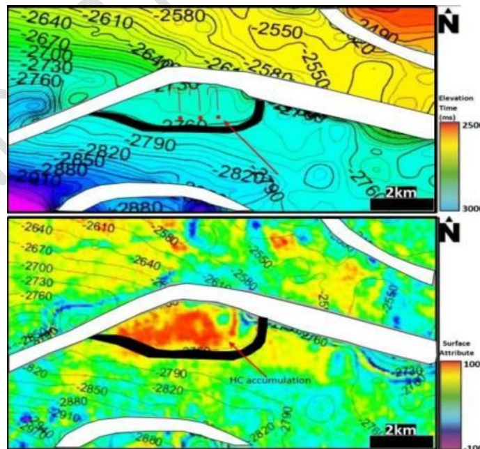
Fig. 9. (a) Time surface map of a horizon mapped at time 2388 with a series of faults dipping in the SW-NE direction. (b) The spectral decomposition map extracted from the OpendTect software. It shows a bright spot region enclosed in a red circle, closing against faults .
