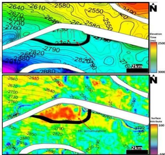
Fig. 840. (a) Interpreted time surface map of a horizon mapped at 2748 showing faults. (b) Contour 2760 is closing on a major fault. The hydrocarbon-bearing region was evident on this
