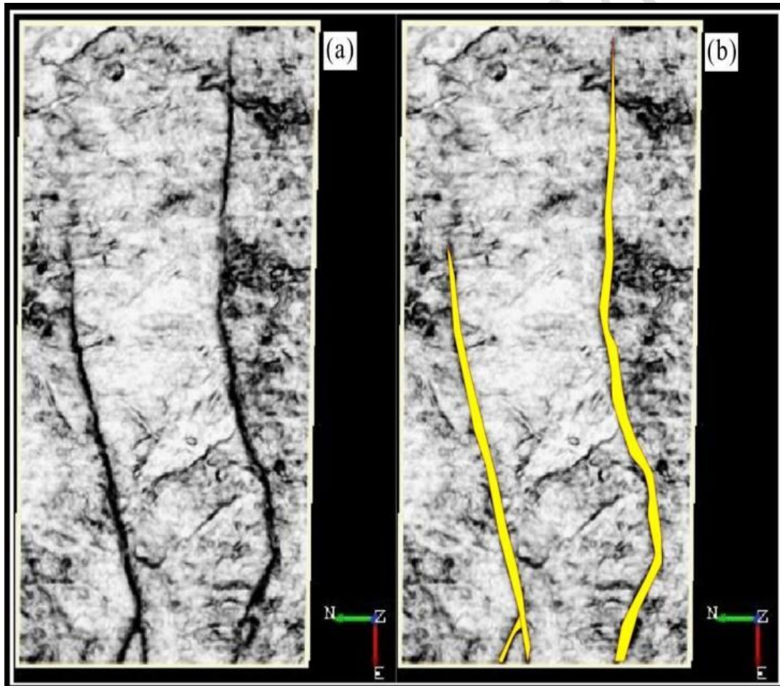
Fig. 6. Extracted similarity attribute maps from inline 5860. (a) shows the uninterpreted map with regions of possible discontinuous reflections. (b) shows the same map with the interpreted faults.
