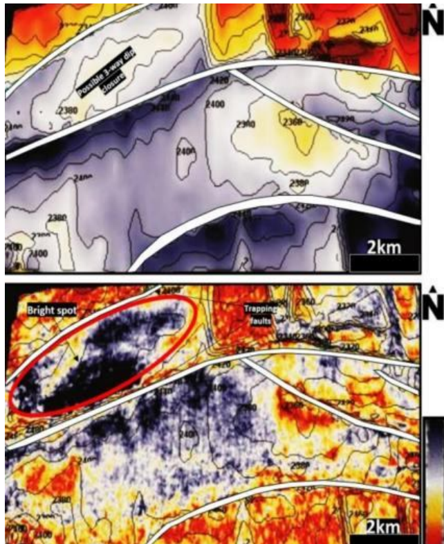
Fig. 910. (a) Time surface map of a horizon mapped at time 2388 with a series of faults dipping in the SW-NE direction. (b) The spectral decomposition map extracted from the Opentect software. It shows a bright spot region enclosed in a red circle, closing against faults SUGGESTION – INCLUDE THE EXTRACTED ENERGY ATTRIBUTE MAP AT SAME SURFACE IN ORDER TO COMPARE WITH SPECTRAL DECOMPOSITION MAP AND COMMENT.
