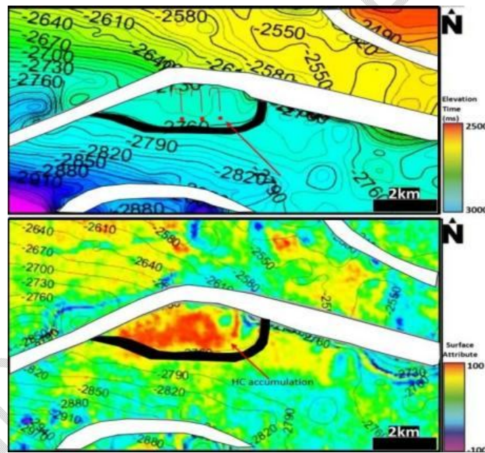
Fig. 408. (a) Interpreted time surface map of a horizon mapped at 2748 showing faults. (b) Contour 2760 is closing on a major fault. The hydrocarbon-bearing region was evident on this attribute map in contour 2760 of the surface map in (a). HC stands for hydrocarbon accumulation
