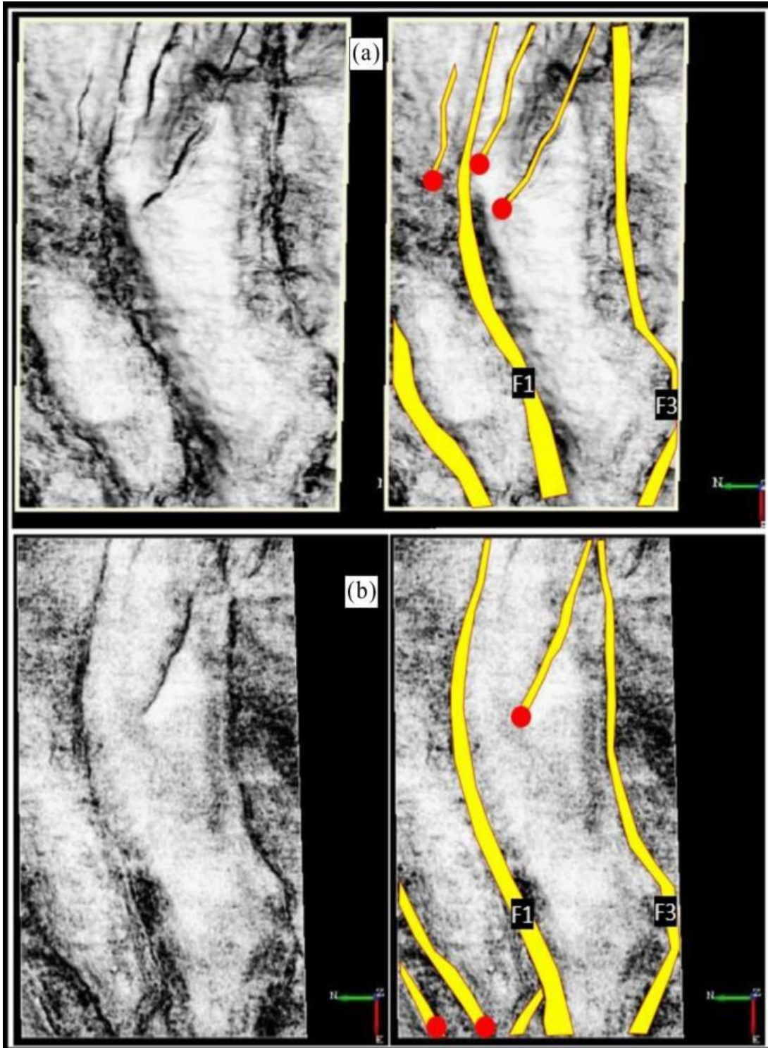
Fig. 7. Extracted similarity attribute maps from inlines 5884(a) and 5980(b). On the left of both (a) and (b) are the uninterpreted maps showing regions of possible discontinuous reflections. On the right are the same map with the interpreted faults. F1 and F3 represent fault one and fault three, respectively. The red circles are placed on faults not identified on the seismic sections. WHERE ARE FAULTS F4 AND F5 INTERPRETED IN THE SEISMIC LINES (Fig. 5)
