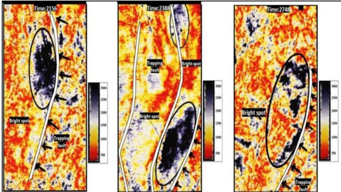
Fig. 89. Time slices showing areas of high amplitude anomalies observed at times 2156, 2388 and 2748, respectively. Using energy attributes, these areas are interpreted as bright spots (potential hydrocarbon areas), and hydrocarbon accumulation was observed to close up on faults.
