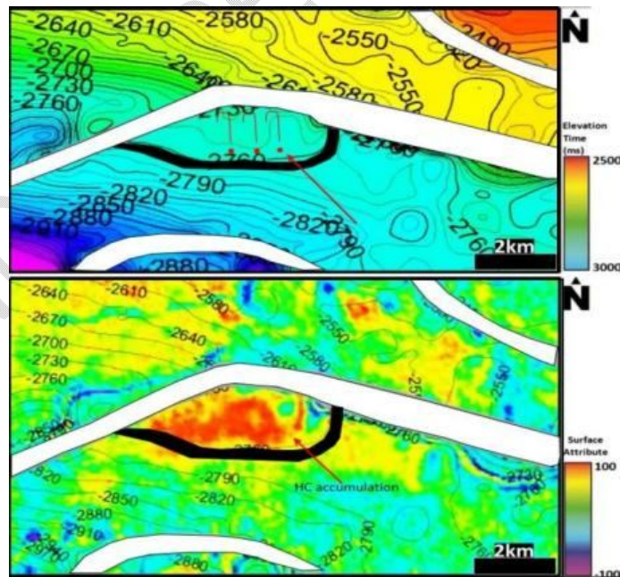
Fig. 10. (a) Interpreted time surface map of a horizon mapped at 2748 showing faults. (b) Contour 2760 is closing on a major fault. The hydrocarbon-bearing region was evident on this attribute map in contour 2760 of the surface map in (a). HC stands for hydrocarbon accumulation
