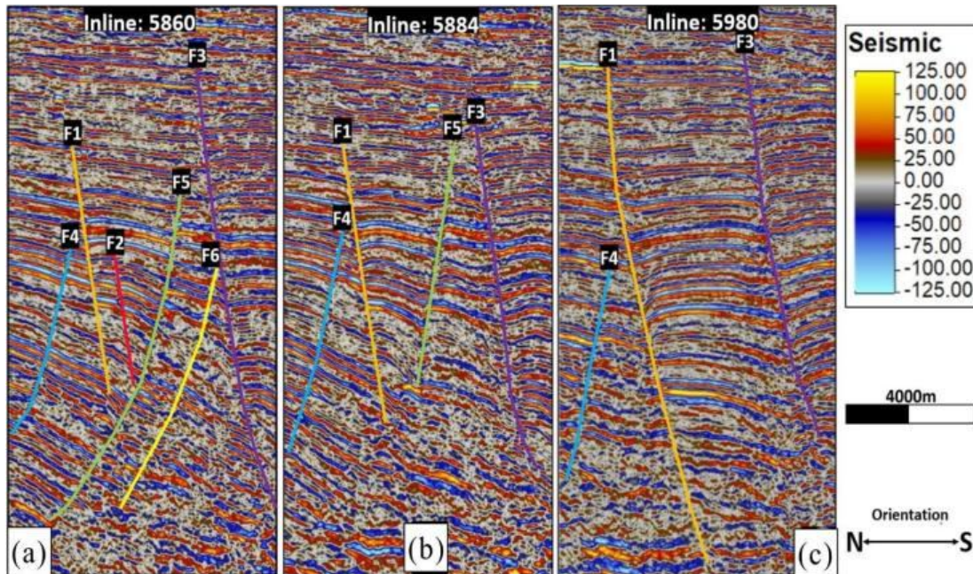
Fig. 5. Interpreted seismic sections of in-lines 5860, 5884, and 5980. Six faults were observed and interpreted on seismic sections A, B and C
