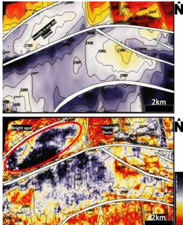
Fig. 9. (a) Time surface map of a horizon mapped at time 2388 with a series of faults dipping in the SW-NE direction. (b) The spectral decomposition map extracted from the OpendTect software. It shows a bright spot region enclosed in a red circle, closing against faults
