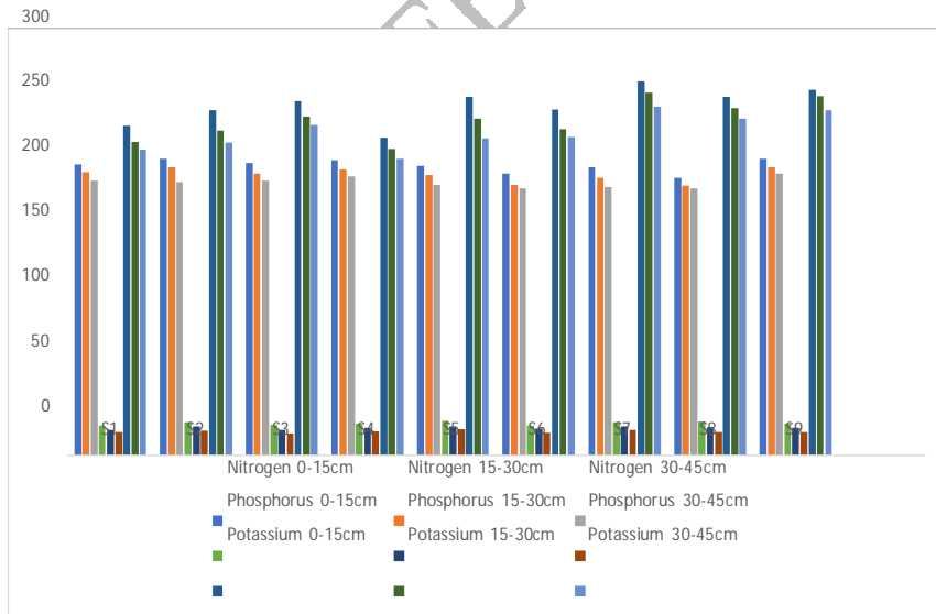
Fig 3: Available Nitrogen, Available Phosphorous and Available Potassium
