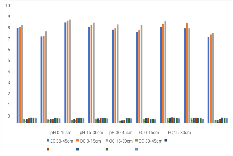
Fig 2: pH, EC and Organic Carbon
