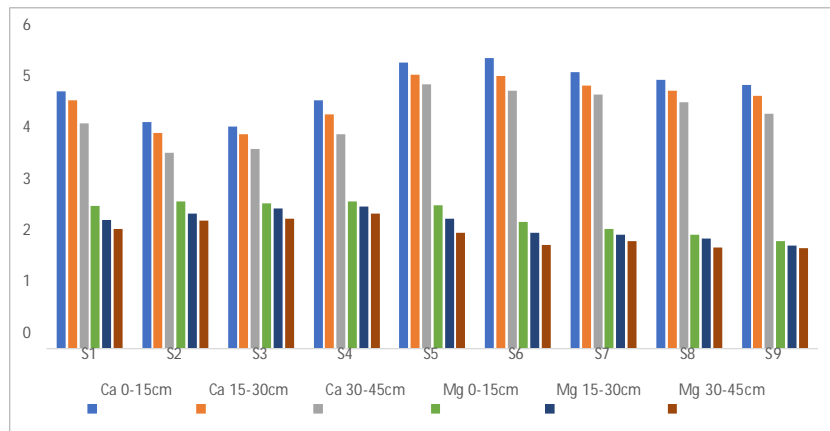
Fig 4: Exchangeable Calcium and Magnesium [meq 100g -1 ]
