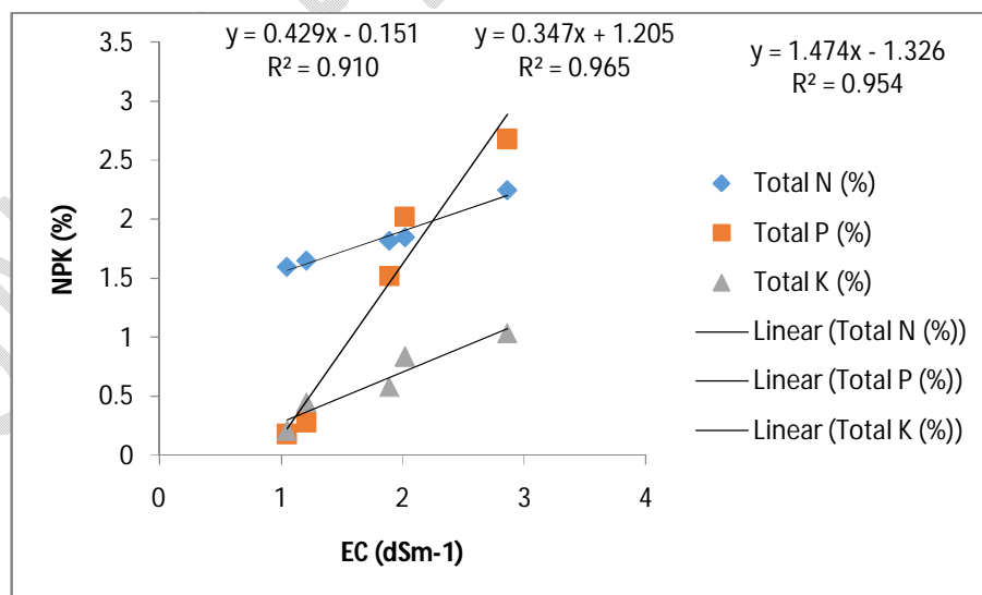
Fig.6. Correlation between Electrical Conductivity and NPK content
