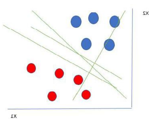
Figure 2 – SVM Hyperplane
