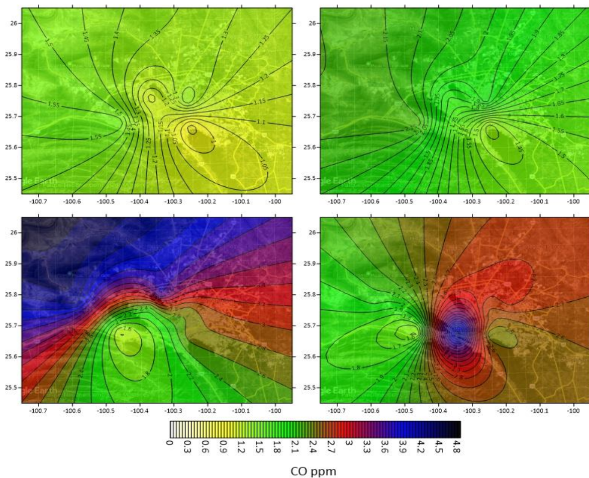
Fig. 22 Temporal space distribution for the highest month of CO (ppm) in the MMA (years a) 2000, b) 2005, c) 2010 and d) 2014.
