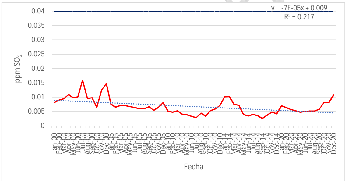
Fig. 15 Monthly average of SO 2 in ppm in the MMA (years 2000, 2005, 2010, 2014 and 2020)
