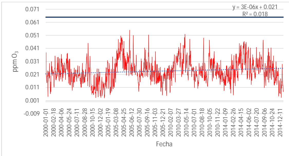
Fig. 11 Daily average of O 3 in ppm in the MMA (years 2000, 2005, 2010 and 2014 )
