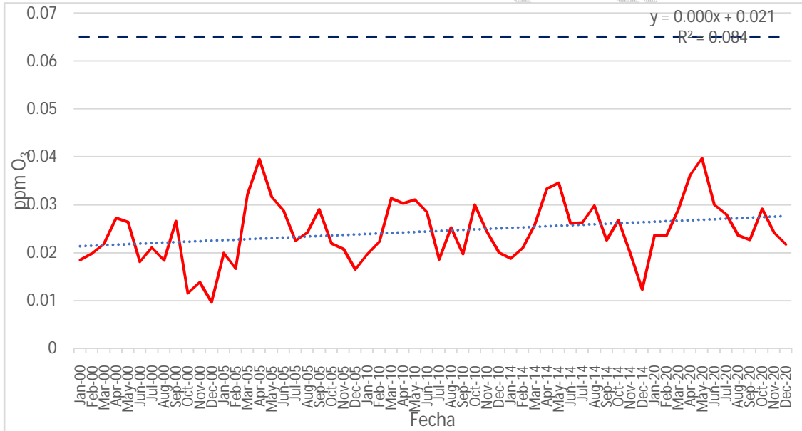
Fig. 12 Monthly average of O 3 in ppm in the MMA (years 2000, 2005, 2010, 2014 and 2020)
