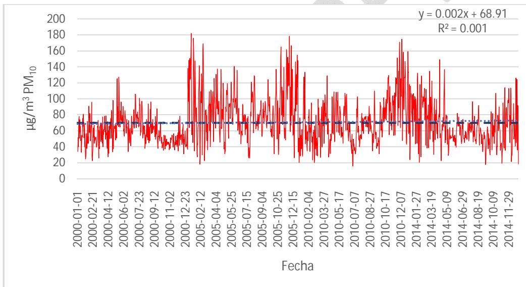
Fig. 5 Daily average of PM 10 in \mu\text{g}/\text{m}^3 in the MMA (years 2000, 2005, 2010 and 2014)
