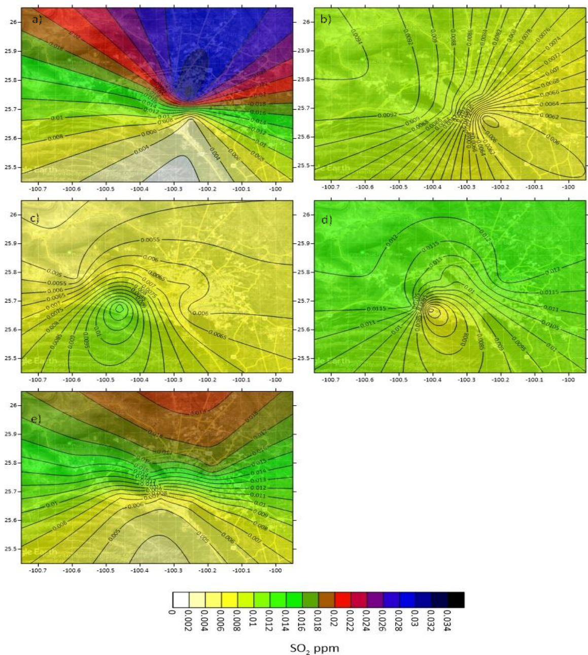
Fig. 16 Temporal space distribution for the highest month of SO 2 (ppm) in the MMA (years a) 2000, b) 2005, c) 2010, d) 2014 and e) 2020).
