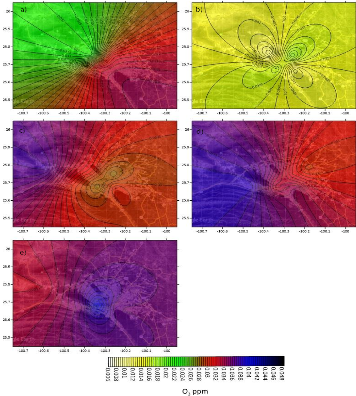
Fig.13 Temporal space distribution for the highest month of O 3 (ppm) in the MMA (years a) 2000, b) 2005, c) 2010, d) 2014 and e) 2020).
