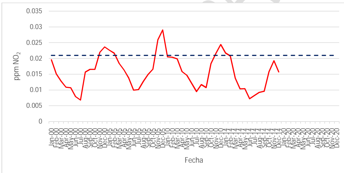
Fig. 18 Monthly average of NO 2 in ppm in the MMA (years 2000, 2005, 2010 and 2014)
