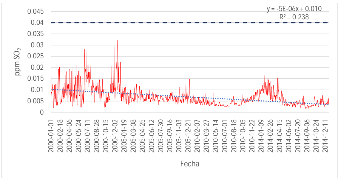
Fig. 14 Daily average of SO 2 in ppm in the MMA (years 2000, 2005, 2010 and 2014)
