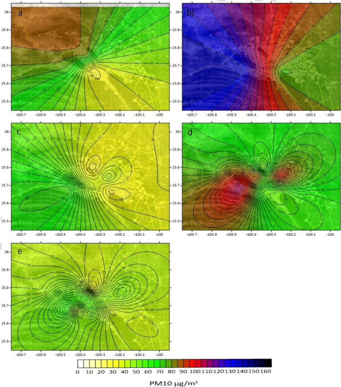
Fig. 6 Monthly average of PM 10 in µg/m 3 in the MMA (years 2000, 2005, 2010, 2014 and 2020).
