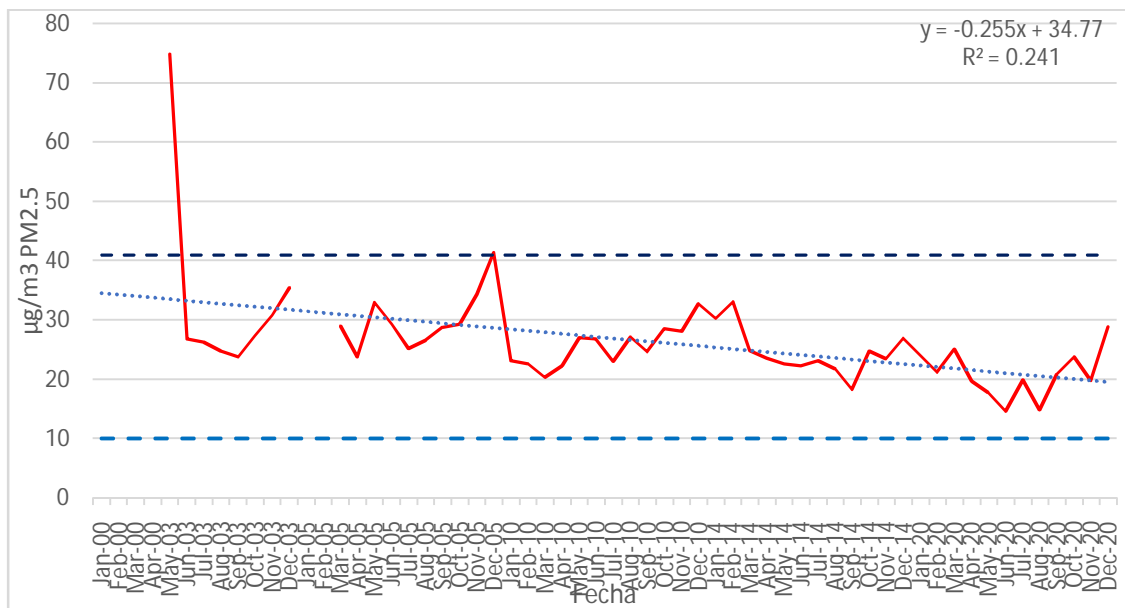
Fig. 9 Monthly average of PM 2.5 in µg/m 3 in the MMA (years 2000, 2005, 2010, 2014 and 2020)
