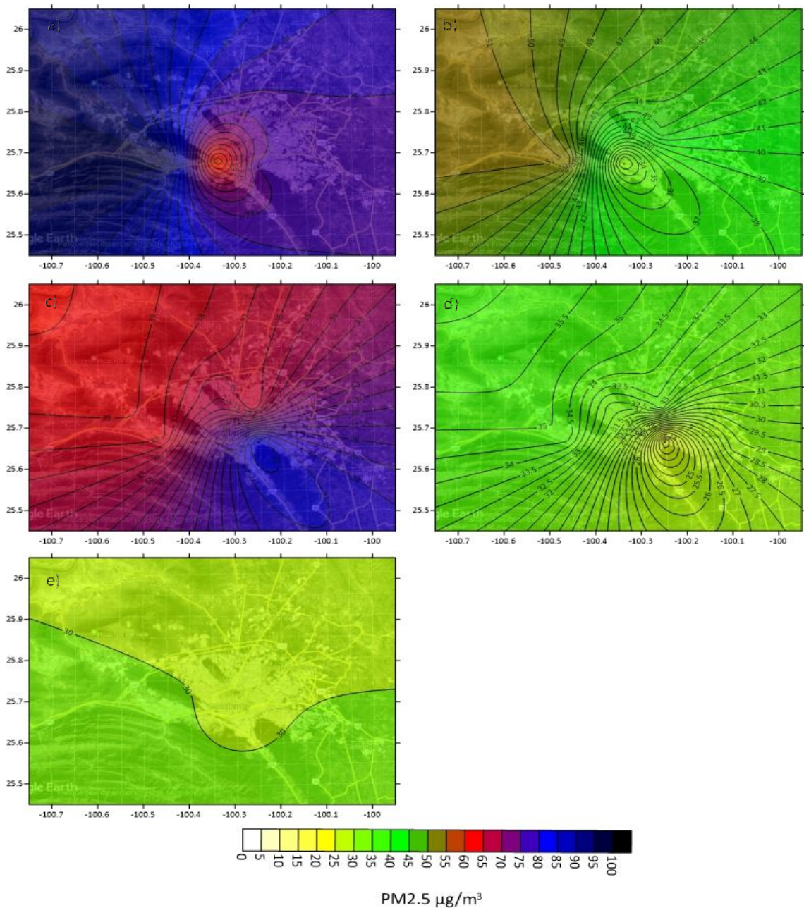
Fig. 10 Temporal space distribution for the highest month of PM 2.5 (µg/m 3 ) in the MMA years a) 2000, b) 2005, c) 2010, d) 2014 and e) 2020).
