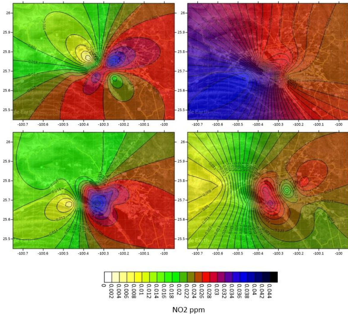
Fig. 19 Temporal space distribution for the highest month of NO 2 (ppm) in the MMA (years a) 2000, b) 2005, c) 2010 and d) 2014.
