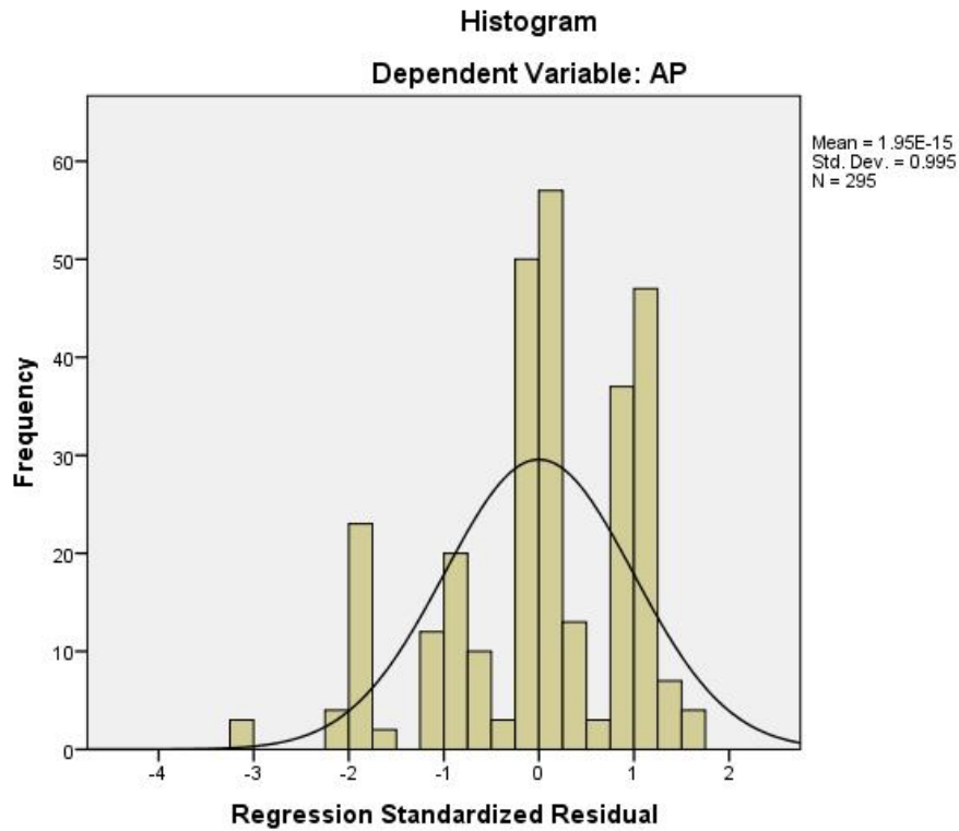
Figure 1: Histogram Normality Test
