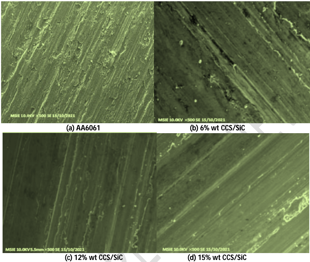
Figure 4: SEM of the worn surfaces of composites with nSiC/nCCSp at 50N, 2.0m/s and 400mm.
