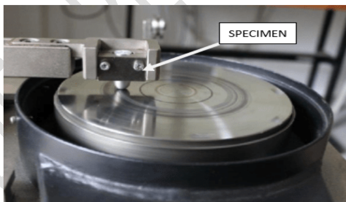
Figure 1 Wear test experimental setup
