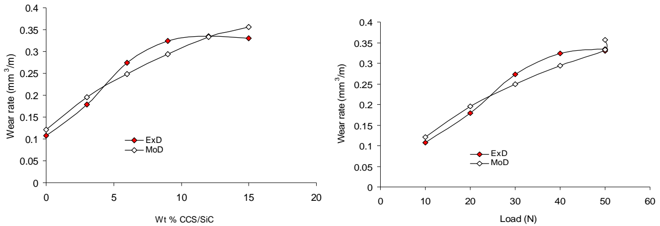
Figure 8: Variation of experimental and model wear rates with (a) concentration of CCS/SiC (b) loading of composites.
