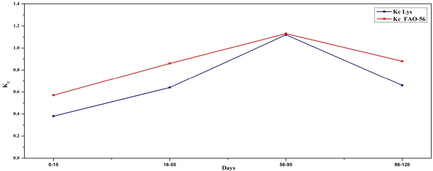
Fig. 2a. Crop coefficients recommended by FAO56 for the crop ( K_c FAO) and determined by lysimeter ( K_c Lys) during rabi season
