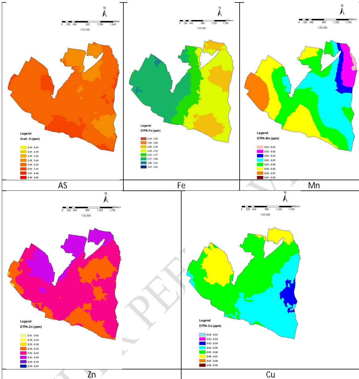
Figure 3. Map of spatial distribution for eleven soil properties in the study area. EC: soil electrical conductivity; SOC: soil organic carbon AN: available nitrogen; AK: available potassium; AP: available phosphorous AS: Available Sulphur;; Fe, Zn, Mn and Cu are DTPA extractable iron, zinc, manganese and copper in soil
