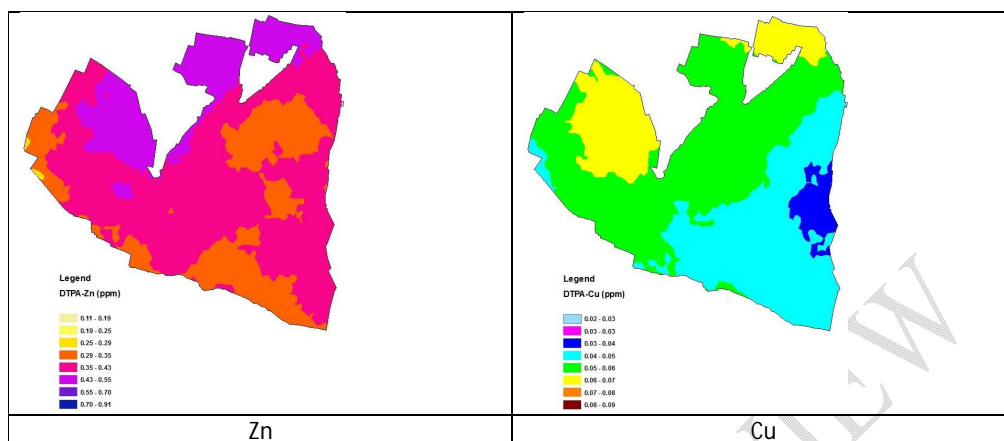
Figure 3. Map of spatial distribution for eleven soil properties in the study area. EC: soil electrical conductivity; SOC: soil organic carbon AN: available nitrogen; AK: available potassium; AP: available phosphorous AS: Available Sulphur; Fe, Zn, Mn and Cu are DTPA extractable iron, zinc, manganese and copper in soil
