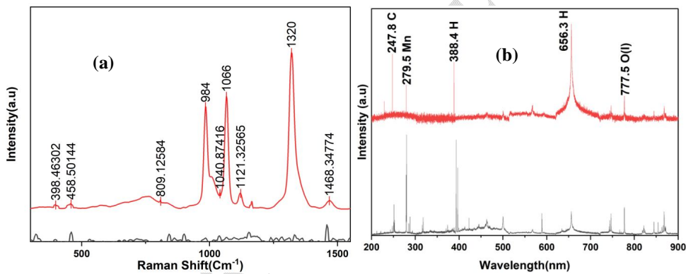
Figure 3:(a) Raman spectra and (b) LIBS spectra for samples containing PP
