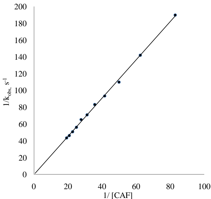
Figure 3: Michealis–Mentens plot of 1/k_1 versus 1/[CAF] at [MnO_4^-] = 2.0 \times 10^{-4} \text{ moldm}^{-3} , [CAF] = (1.20 - 5.20) \times 10^{-2} \text{ moldm}^{-3} , I = 0.5 \text{ moldm}^{-3} ( Na_2SO_4 ) and T = 24.0 \pm 0.1^\circ\text{C} .
