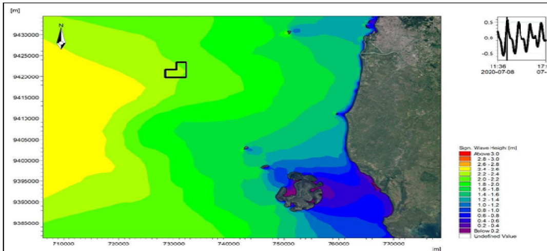
Figure 3. Overview of wave height at high tide in the east season
