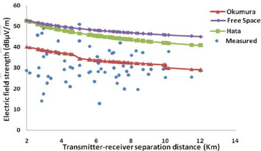
Figure 1.: Comparison of the Measured and Predicted Field Strength of NTA Yenagoa
