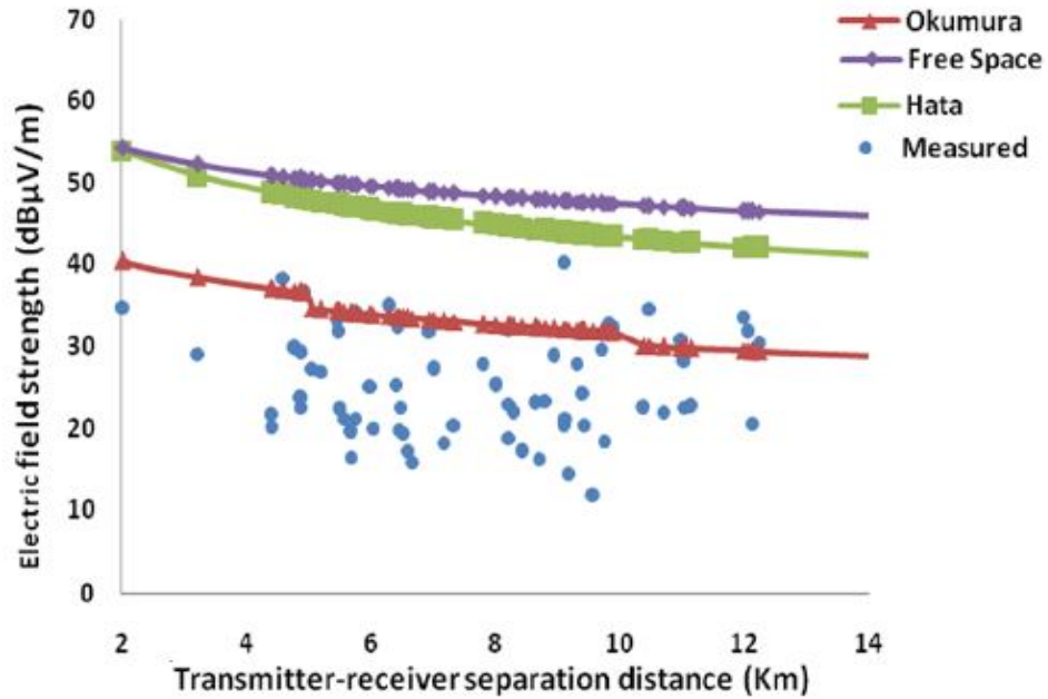
Figure 2.: Comparison of the Measured and Predicted Field Strength of NDTV
