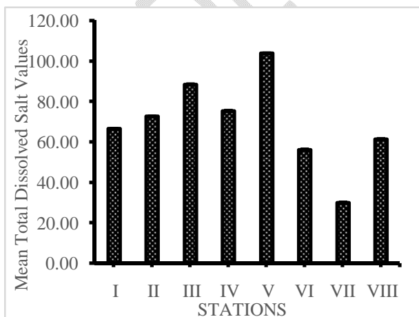
Fig 6: Mean Total Dissolved Salt Values of Swamp Ponds in Engenni
