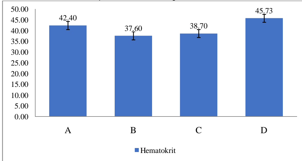
Figure 1. Hematocrit Value of Biawan Fish
