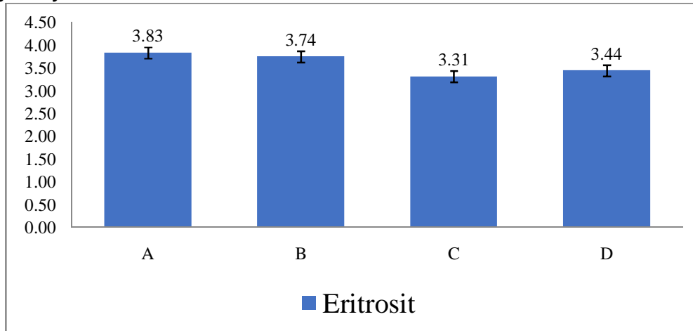
Figure 2. Erythrocyte Value of Biawan Fish ( x 10 6 / μL )
