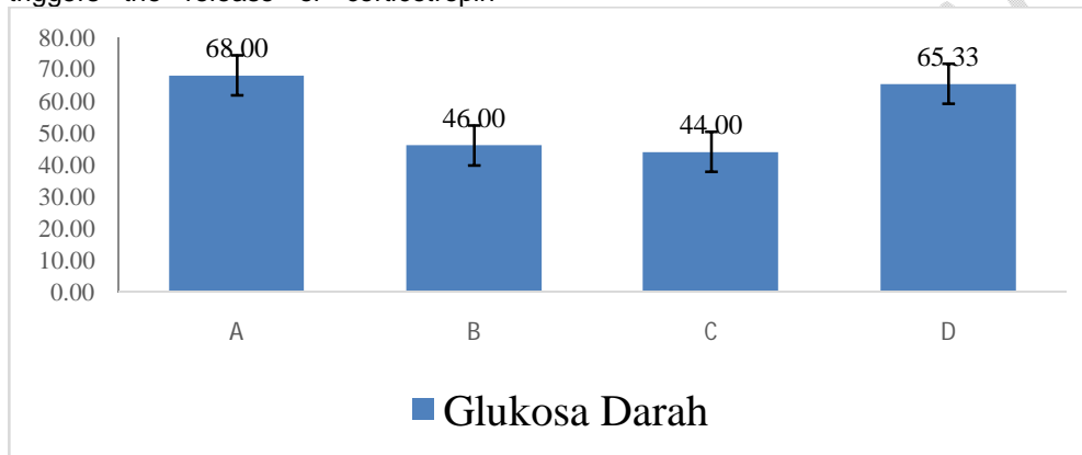
Figure 3. Biawan Fish Blood Glucose Value (mg/dL)
