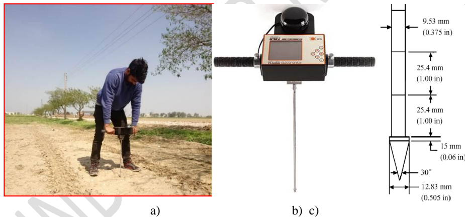
Fig. 1 Measurement of cone index using hand operated cone penetrometer a) Field view, b) Used cone penetrometer (RIMIK CP40II) and c) Standard dimensions of penetrometer
