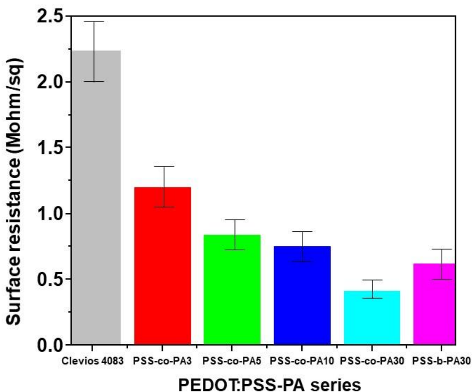
Figure 4. Sheet resistance of Clevios 4083 and PEDOT:PSS-PA films.
