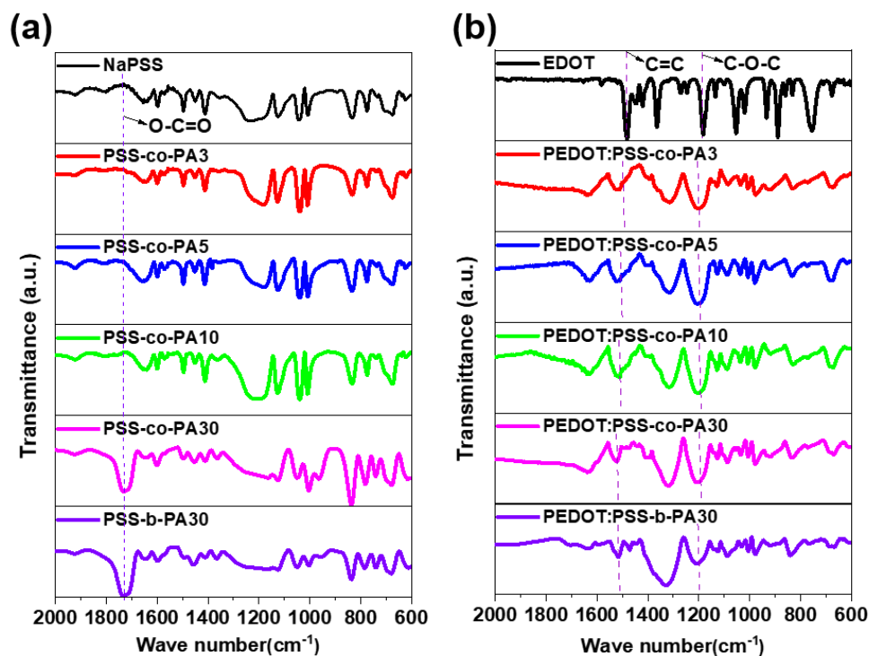
Figure 2. FT-IR spectra of NaPSS and PSS-PA series, and PEDOT:PSS-PA complexes.
