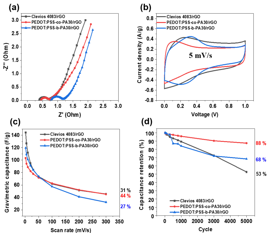
Figure 8. Electrochemical performances of the Clevios 4083/rGO, PEDOT:PSS-co-PA30/rGO and PEDOT:PSS-b-PA30/rGO aerogels. (a) Nyquist plots, (b) CV curves at the scan rate of 5 \text{ mV s}^{-1} , (c) Specific capacitances with scan rates ranging from 5 to 300 \text{ mV s}^{-1} , (d) Cyclic stability at the scan rate of 100 \text{ mV s}^{-1} .
