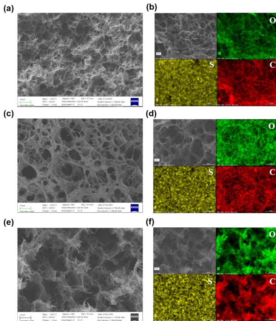
Figure 7. Low-magnification FESEM images of (a) Clevios 4083/rGO aerogel, (c) PEDOT:PSS-co-PA30/rGO aerogel, and (e) PEDOT:PSS-co-PA30/rGO aerogel; SEM image and elemental mappings of C, O and S of (b) PEDOT:PSS/rGO aerogel, (d) PEDOT:PSS-co-PA30/rGO aerogel, (e) PEDOT:PSS-co-PA30/rGO aerogel.
