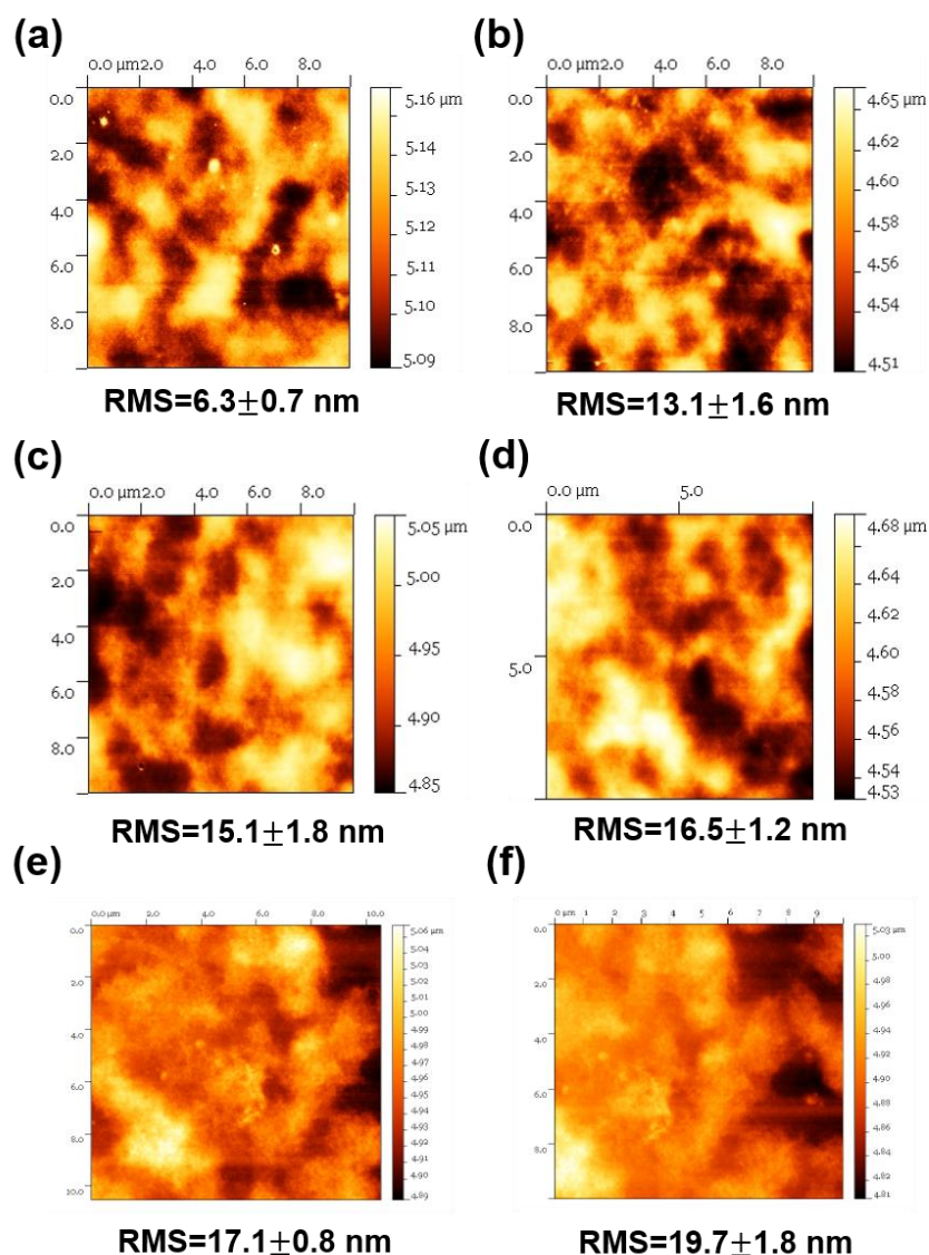
Figure 6. AFM topography images of (a) Clevios 4083, (b) PEDOT:PSS-co-PA3, (c) PEDOT:PSS-co-PA5, (d) PEDOT:PSS-co-PA10, (e) PEDOT:PSS-co-PA30, (f) and PEDOT:PSS-b-PA30 films;
