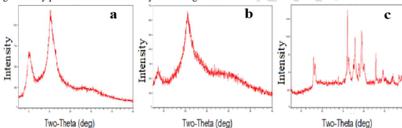
Figure 4. XRD diffractograms of a = CS, b = PCAFC and c = PCAFC-Cu(II) (Source of a and b : [17]).
