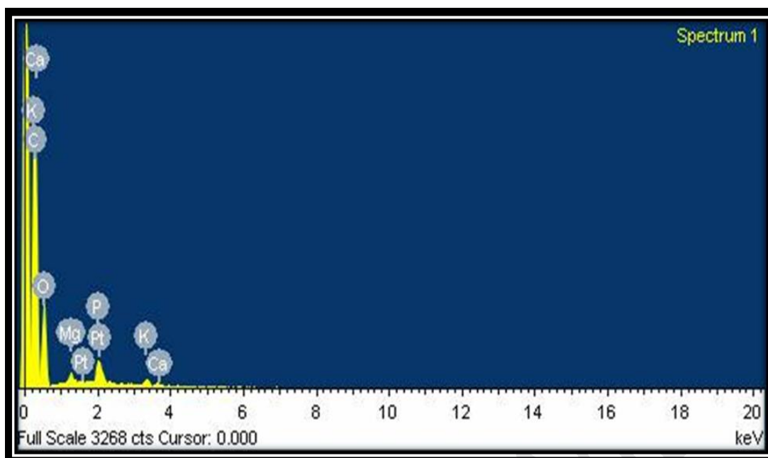
Figure 2. EDX graph of the product
