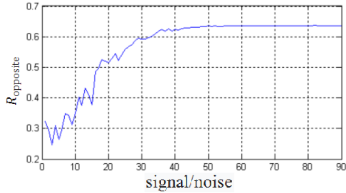
Figure 1. Dependence of R_{\text{opposite}} on the signal-to-noise ratio.
