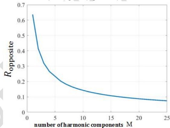
Figure 3. Dependence of the required support level R_{\text{opposite}} on the number of harmonic components.
