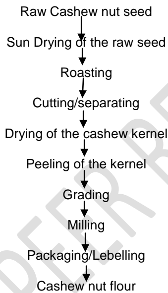
Fig. 2. Flow Process for the Production of Cashew nut flour
