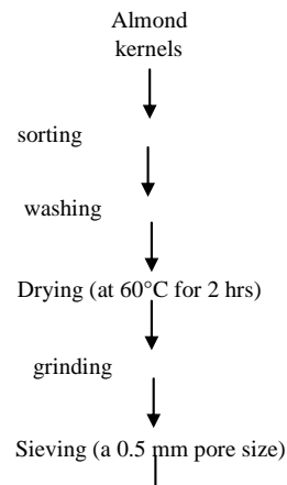
Figure 2: Flow chart for the production of almond kernel flour Source: (Guyihet et al. , 2020)
