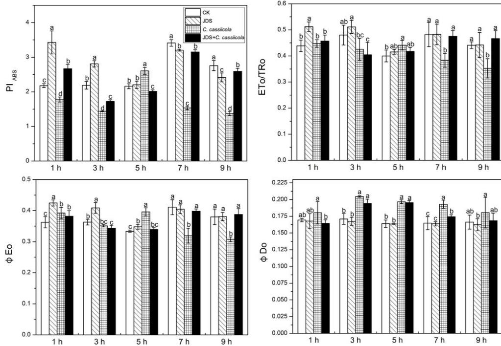
Fig. 2 Effects of JDS on F_0 , F_m , \phi P , F_v/F_0 , D_{lo}/CSO , RC/CSO , TRo/CSO , ETo/CSO , PI_{ABS} , \phi_o , \phi E_o and \phi Do under the stress of C.cassicola
