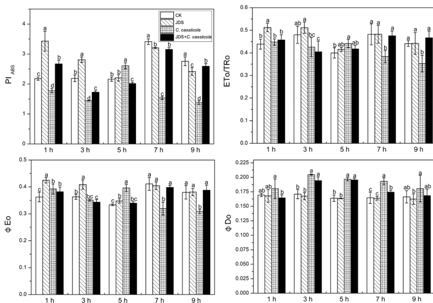
Fig. 2 Effects of JDS on F 0 , F m , φ P , F v /F 0 , D io /C SO , R C /C SO , T Ro /C SO , E To /C SO , P I ABS , φ o , φ Eo and φ Do under the stress of C. cassiicola
