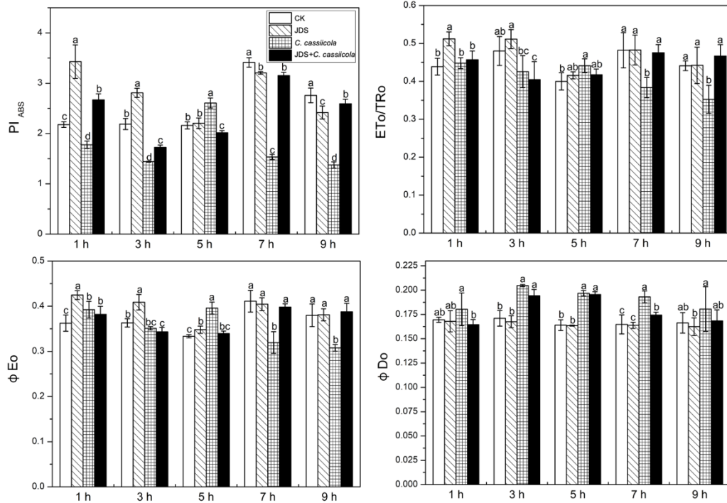
Fig. 2 Effects of JDS on F_0 , F_m , \phi P , F_v/F_0 , D_{10}/CSO , RC/CSO , TRo/CSO , ETo/CSO , PI_{ABS} , \phi o , \phi Eo and \phi Do under the stress of C.cassicola
