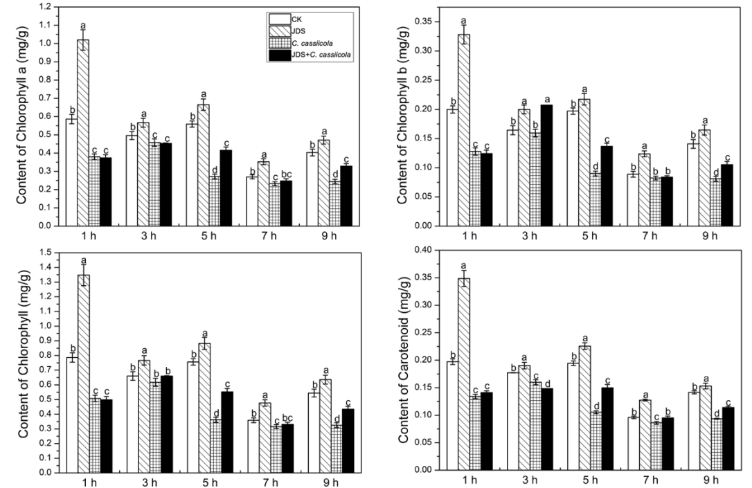
Fig. 1 Effects of JDS on Chl a, Chl b, Chl and Car under C.cassicola stress 3.2 Effect of JDS on chlorophyll fluorescence parameters of cucumber seedlings under C. cassicola stress
