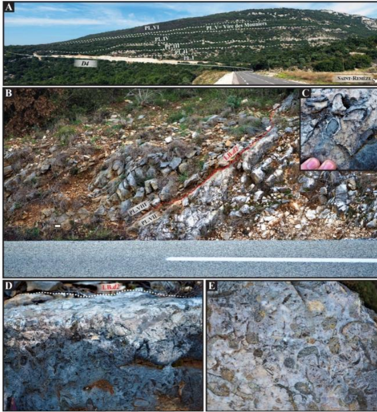
Fig. 7. Field photographs of the Pont de Laval section: (A) Panorama of the lower section showing the PL.I to PL.VI units. (B) Close-up view of the LB.d2 discontinuity atop (C) Agriopleura -rich rudist limestones (Serre de Tourre fauna) of the PL.VII unit, (D) and (E) Details of the prominent hardground of the LB.d2 discontinuity showing bioclastic infilling in rudist shells down to a fringe of several centimetres.
