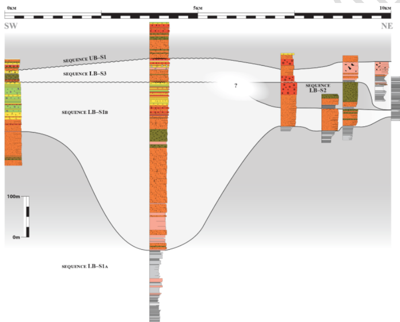
Fig. 13. Platform-to-basin correlations of the Urgonian Bas-Vivarais domain. The LB.d2 discontinuity is used as datum (flattening surface) in this cross section.
