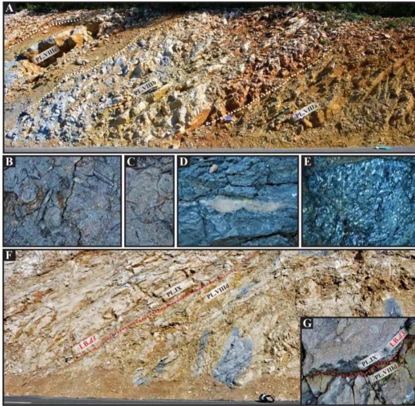
Fig. 8. Field photographs of the Pont de Laval section: (A) Panorama of the upper section showing the first three units of the STB, (B) Close-up view of echinoid and bryozoan remains from obliquely laminated calcarenites of the PL.VIIIa sub-unit, (C) In situ requieniidrudist from the Offneria simplex beds of the PL.VIIIc sub-unit, (D) Platy and (E) branched corals from the PL.VIIId sub-unit, (F) Panorama of the LB.d3 discontinuity atop the STB (PL.VIIId sub-unit), and (G) close-up view of the same discontinuity showing the change from coral-rich oobioclastic to coarse-grained calcarenite sediments.
