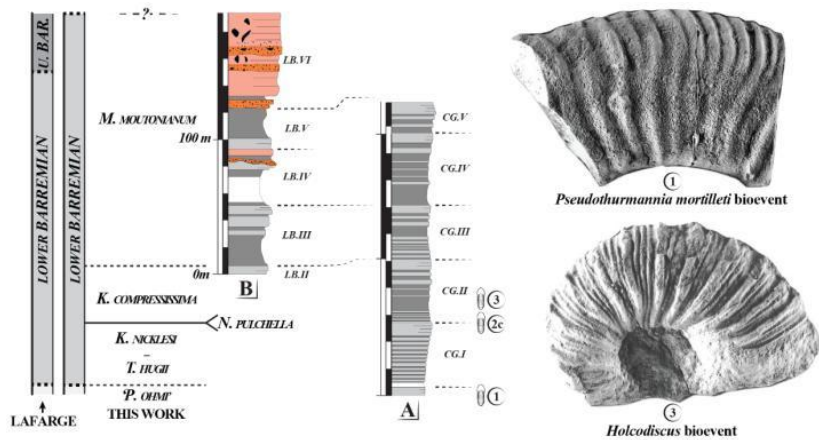
Fig. 11. Lithostratigraphic, sedimentologic and biostratigraphic interpretations of (A) Calvaire de Gras, and (B) Le Bauzu. Acronyms in black refer to the depositional sequences of [2].
