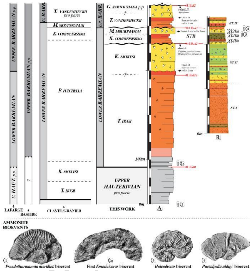
Fig. 4. Lithostratigraphic, sedimentologic and biostratigraphic interpretations of the Serre de Tourre–Chames section (A) after [23] and (B) after thin-section re-examination of [8]. Acronyms in black and red refer, respectively, to the depositional sequences of [2] and remarkable surfaces described in the present contribution. Age assignments are derived from remarkable surfaces of regional significance dated by means of ammonite bioevents figured below (after [23], not to scale). Comparison with previous dating of [2, 8, 23, 31] are added.
