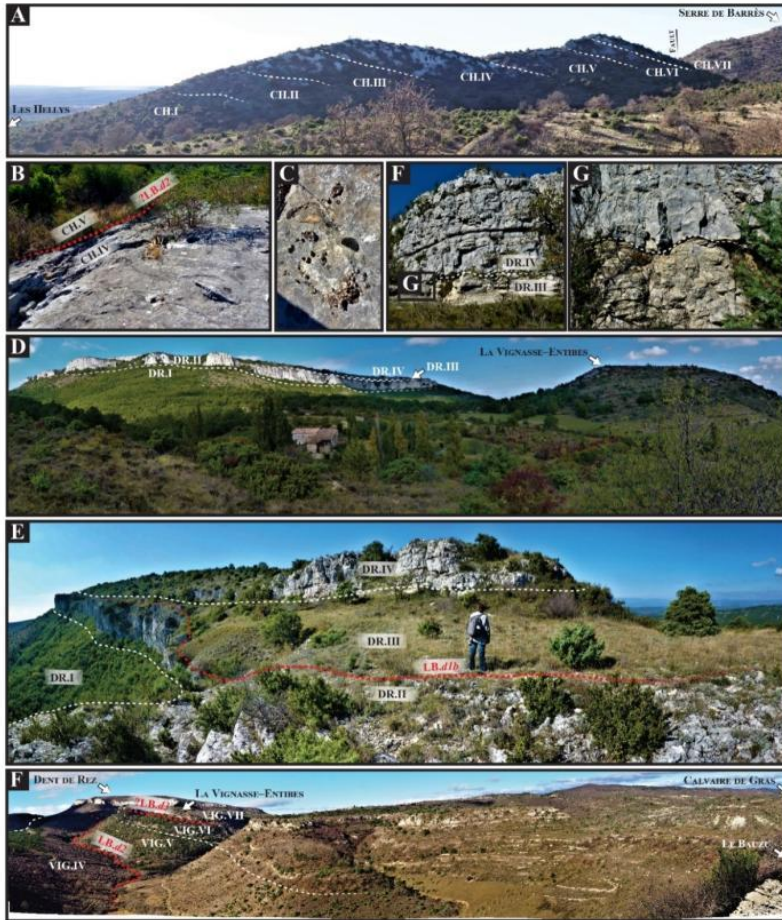
Fig. 10. Field photographs of the Chastellas des Hellys, Dent de Rez, and La Vignasses–Entibes sections: (A) Panorama of the Chastellas des Hellys section showing all the units of [2], (B) Close-up view of the putative LB.d2 discontinuity atop the coral-rich CH.IV unit, (C) Close-up view of siliceous smear at the putative LB.d2 discontinuity sensu [2], (D) Panorama of the Dent de Rez sections, with DR.I to DR.IV units, over Hauterivian–lowermost Barremian hemipelagites, (E) Close-up view of the Gavelinellabarremiana -bearing marlstones (DR.III unit) over the LB.d1b discontinuity. Note the thinning out of the unit in direction of the platform, (F) Close-up view of the echinodermic bioclastic calcarenites of the DR.IV unit at the hilltop of the Dent de Rez section, (G) Close-up view of the wavy base at the base of the DR.IV unit eroding the underlying DR.III marls. (F) Panorama of the Chastellas des Hellys section showing the post-VIG.III units of [2].
