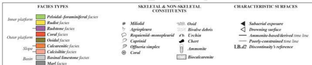
Fig. 2. Facies types, biological–sedimentological symbols and stratigraphic nomenclature used throughout the present contribution Modified after [29]
