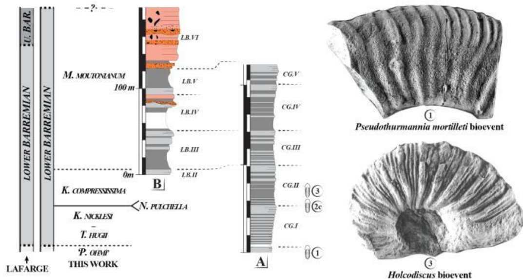
Fig. 11. Lithostratigraphic, sedimentologic and biostratigraphic interpretations of (A) Calvaire de Gras, and (B) Le Bauzu. Acronyms in black refer to the depositional sequences of [2].
