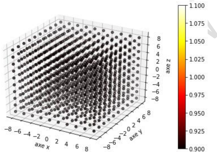
fig5: Graphic representation of the solution set of the first system of inequalities
