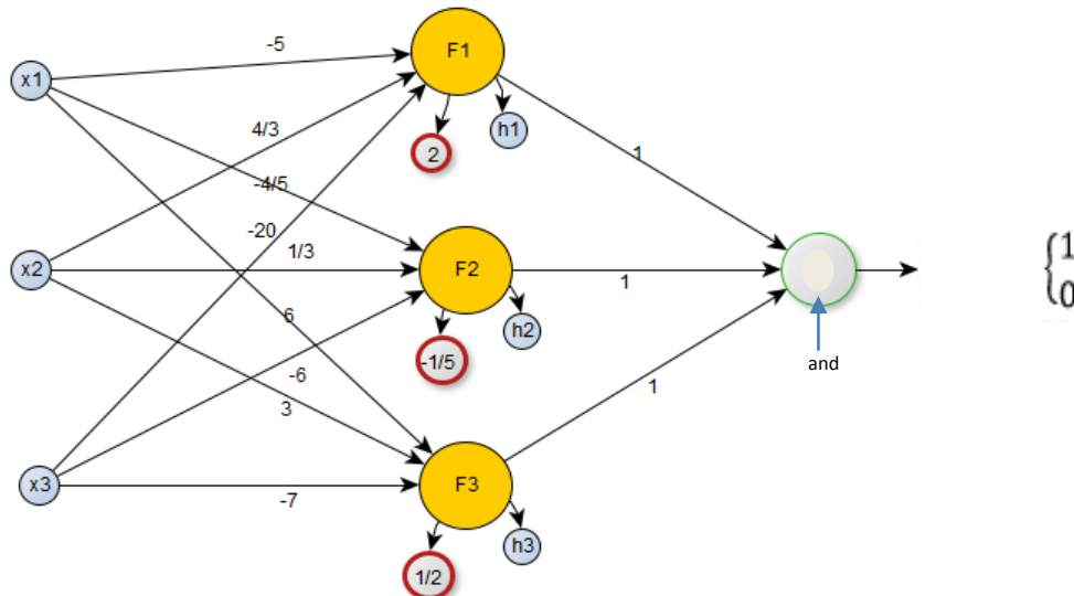
fig8: Neural model of the thirdeexample
