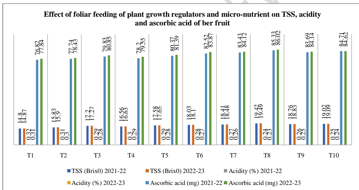
Fig. 1: Effect of foliar feeding of plant growth regulators and micro-nutrient on TSS, acidity and ascorbic acid of ber fruit
