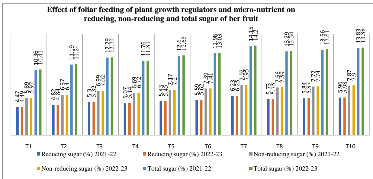
Fig. 2: Effect of foliar feeding of plant growth regulators and micro-nutrient on reducing sugar, non-reducing sugar and total sugar of ber fruit
