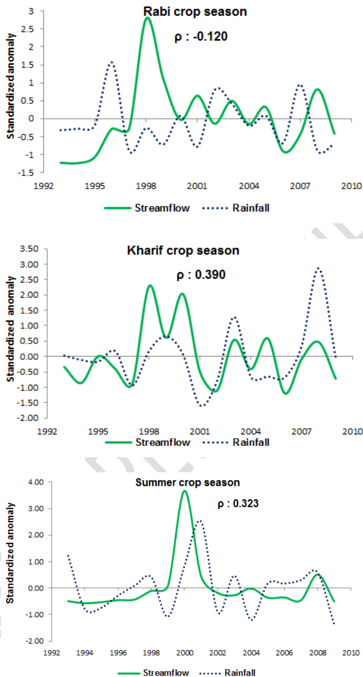
Figure 8. Temporal distribution of standardized anomaly of streamflow and rainfall in different crop season of mid-stream region of Ramganga River basin
