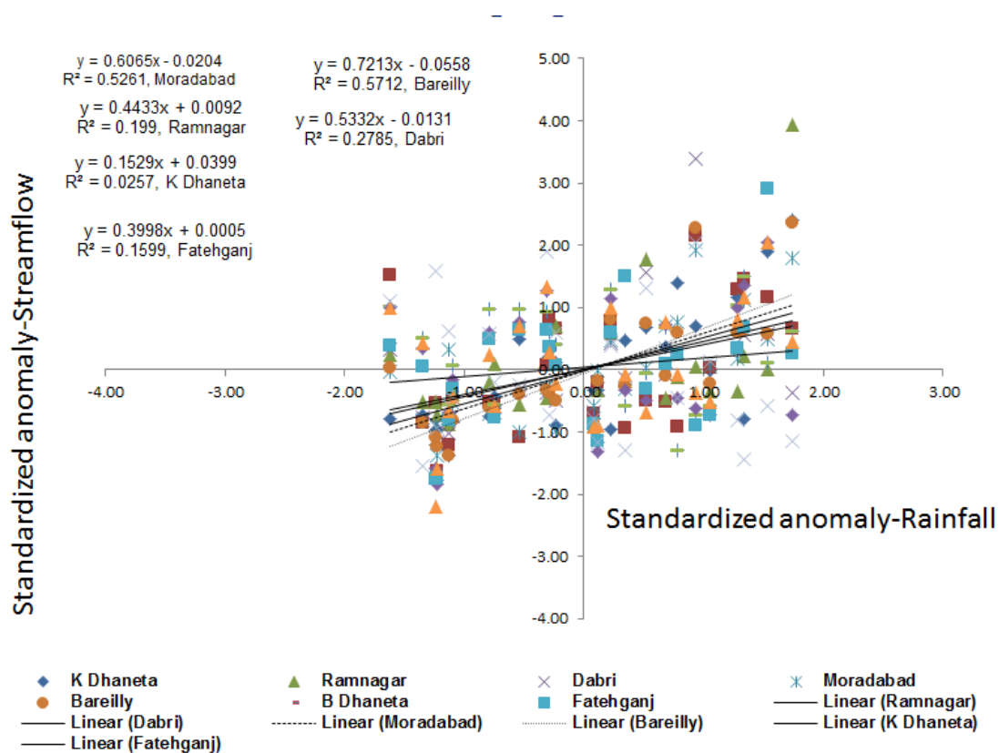
Figure 6. Standardized anomaly of annual streamflows vs rainfall of different catchments of Ramganga River basin
