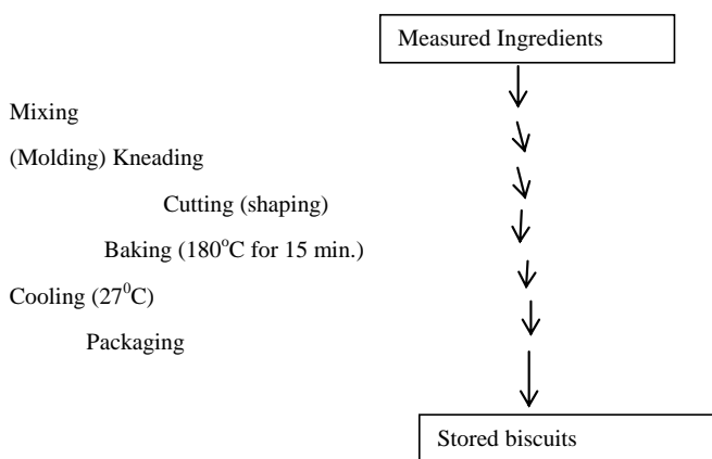
Figure 3. Flow chart for production of biscuits
