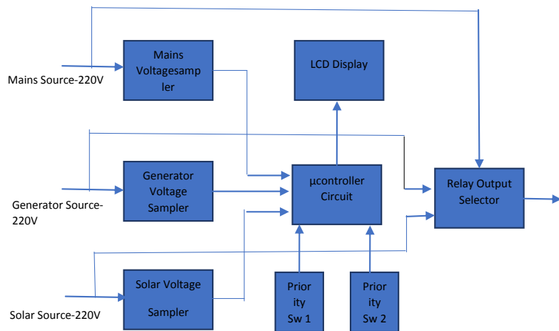
Figure 1: block diagram of the Multiple Source Power Selector
