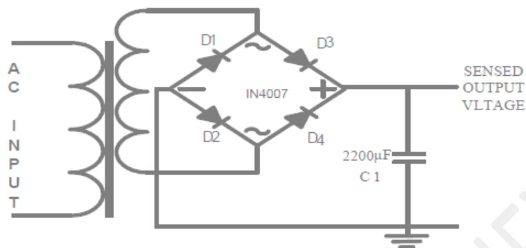
Fig. 2.0: Circuit Diagram of Sensing Unit
