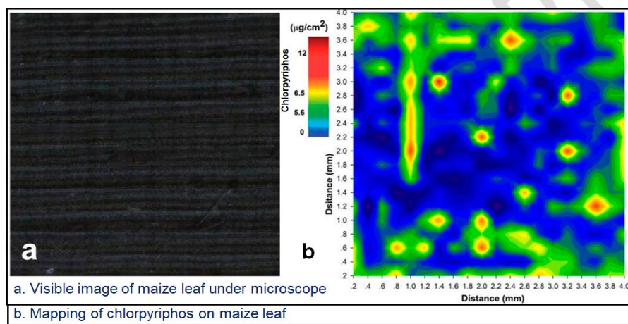
Figure 4. Two dimensional mapping of chlorpyriphos residue on maize leaf
