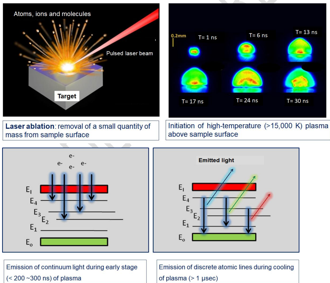
Figure 1. Principle of operation of LIBS
