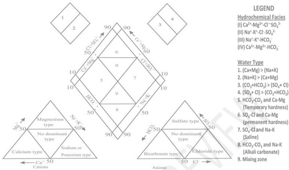
Hydrochemical facies according to Back and Hanshaw, 1965
