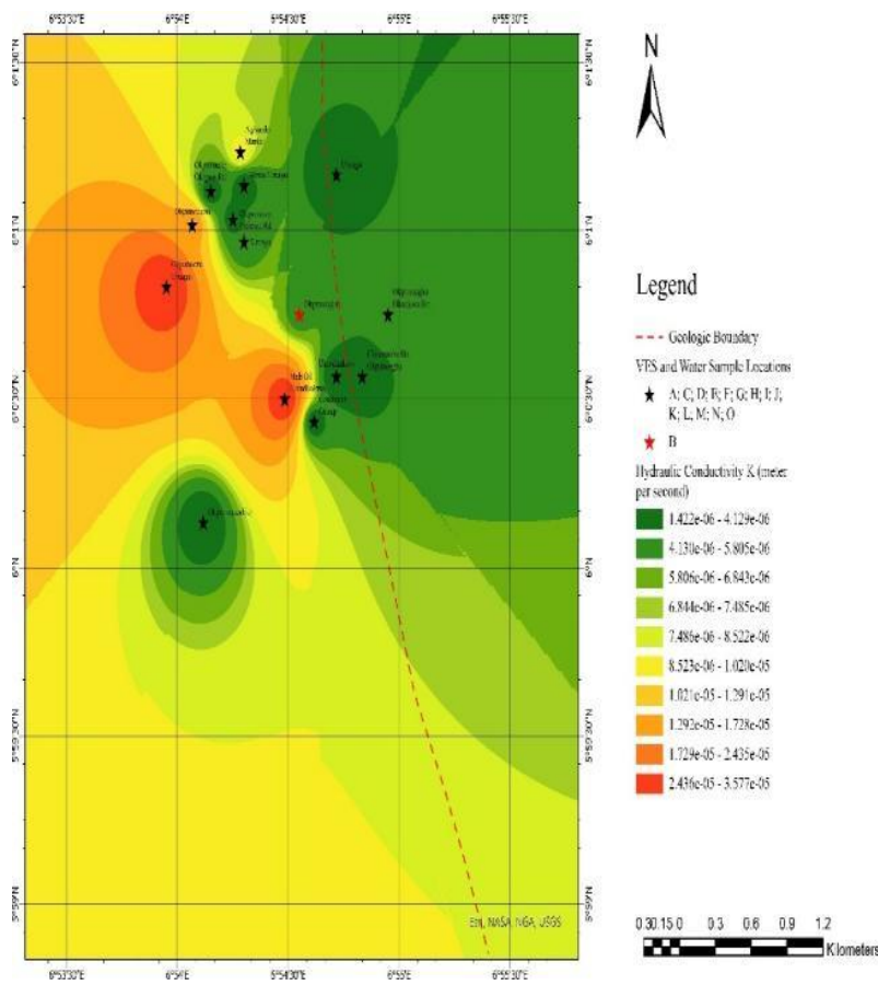
Figure 5: Distribution of K in the study area
