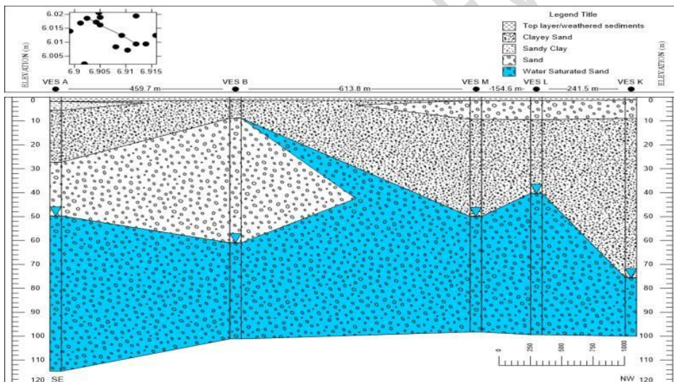
Figure 3: Section made from profile AB correlating strip logs from vertical electrical sounding A, B, M, L and K.
