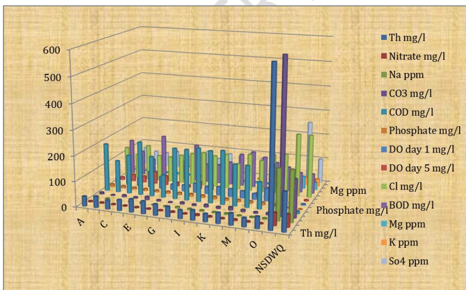
Figure 8: Distribution of the chemical parameter in the water sources with the standards
