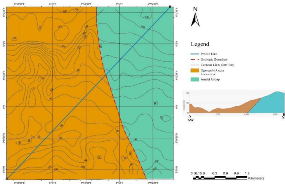
Figure 1: Geology map of study area.
