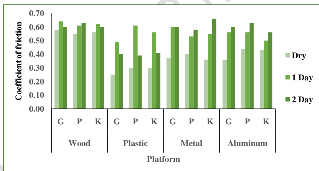
Figure 2: Coefficient of friction under different platforms for different varieties (G- Gavran; P- Puna Fursungi; K- KSP-117)
