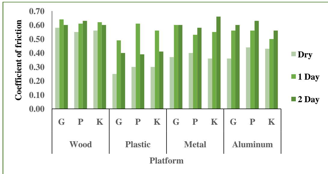
Figure 2: Coefficient of friction under different platform for different varieties (G- Gavran; P- PunaFursungi; K- KSP-117)
