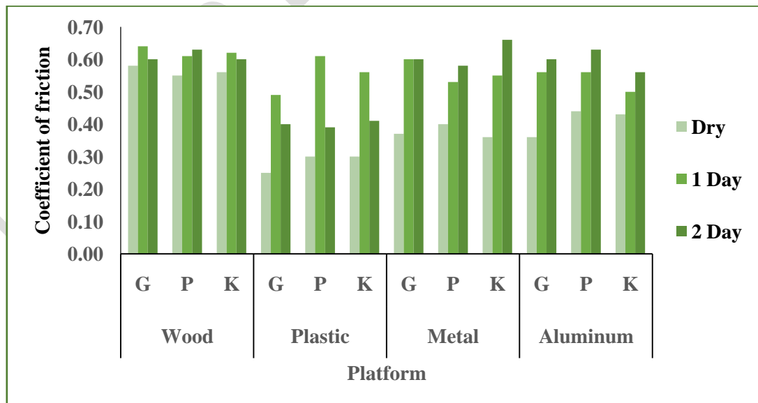
Figure 2: Coefficient of friction under different platform-platforms for different varieties (G- Gavran; P- Puna Fursungi; K- KSP-117)
