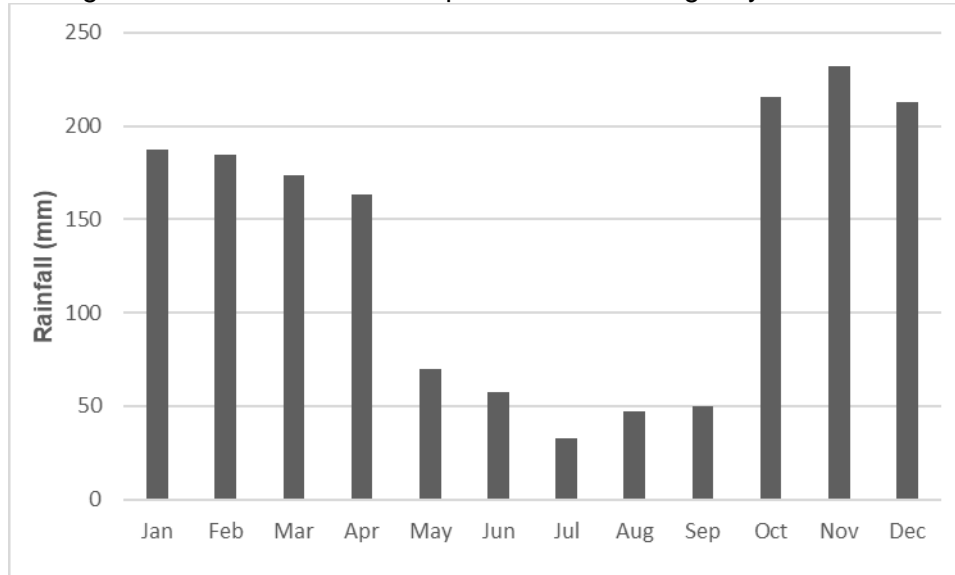
Fig 3. Mundri Rainfall 2018-2022
