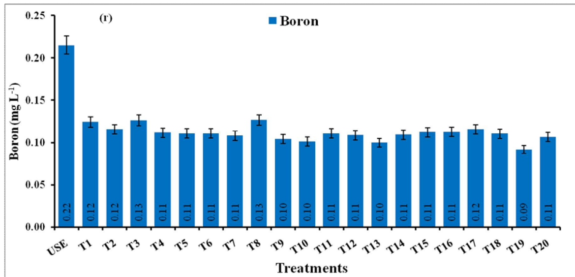
Figure 3: Sewage effluent quality
