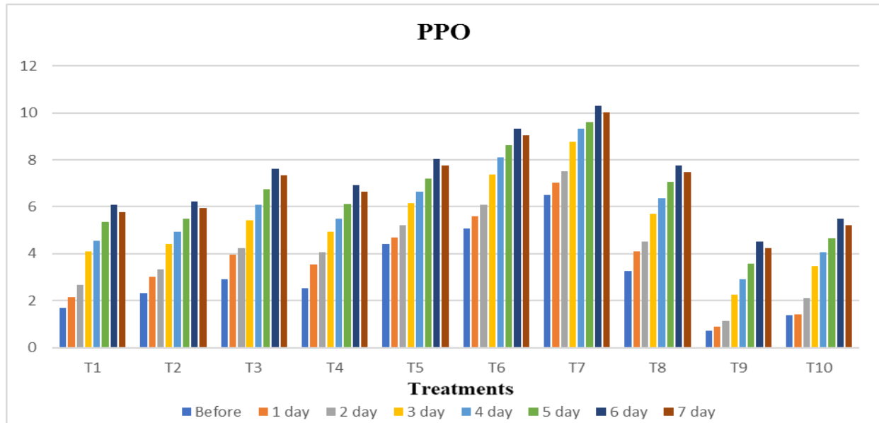
Fig 5. Activity of Polyphenol oxidase(nmoles/min/gm) in different treatments of rice cv. BPT- 5204 in glass house experiment.
