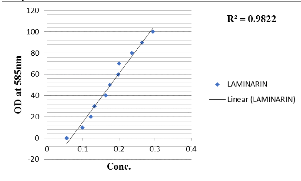
Graph 1. Standard curve of laminarin at 585nm
