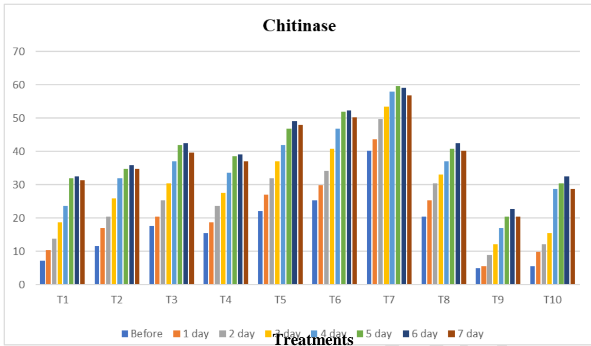
Fig 1. Activity of chitinase ( \mu\text{moles}/\text{min}/\text{gm} ) in different treatments of rice cv. BPT-5204 in glass house experiment.
