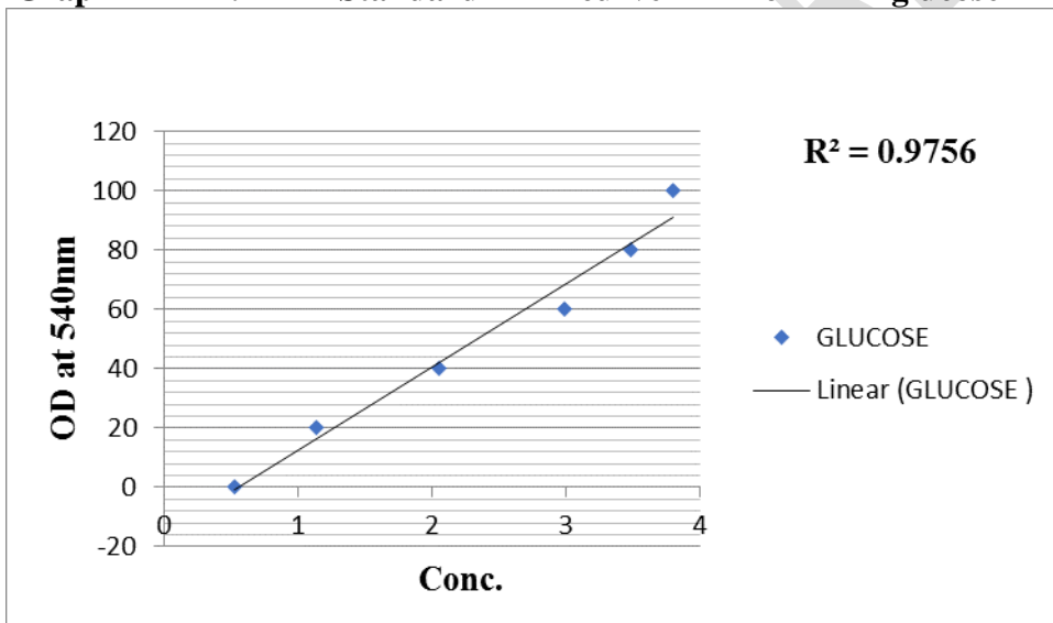
Graph 2. Standard curve of glucose at 540nm
