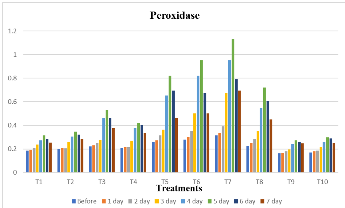
Fig 4. Activity of Peroxidase( \mu\text{moles}/\text{min}/\text{gm} ) in different treatments of rice cv. BPT-5204 in glass house experiment.
