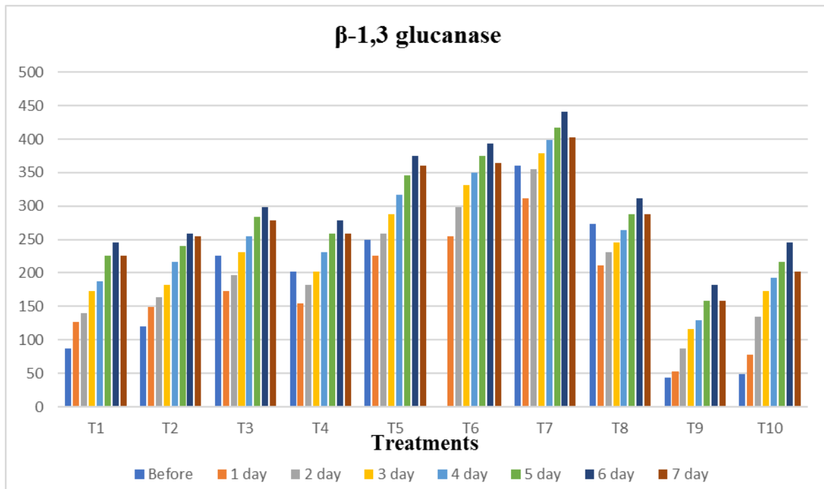
Fig 2. Activity of β-1,3 glucanase (µmoles/min/gm FW) in different treatments of rice cv. BPT- 5204 in glass house experiment.
