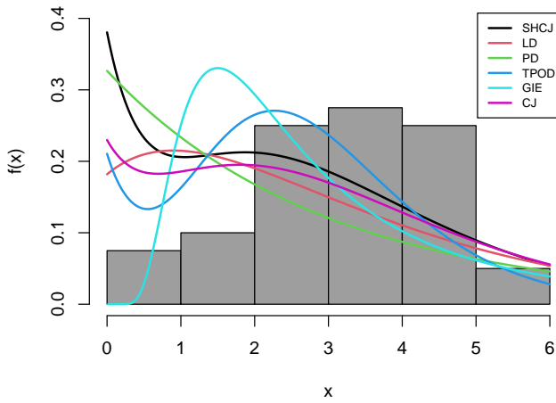
Figure 13: Empirical and Theoretical PDF
