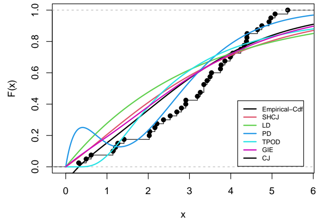
Figure 14: Empirical and Theoretical CDF
