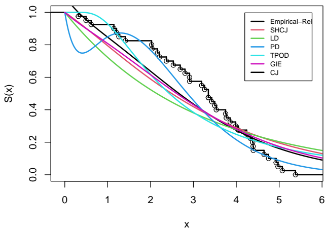
Figure 15: Empirical and Theoretical Reliability
