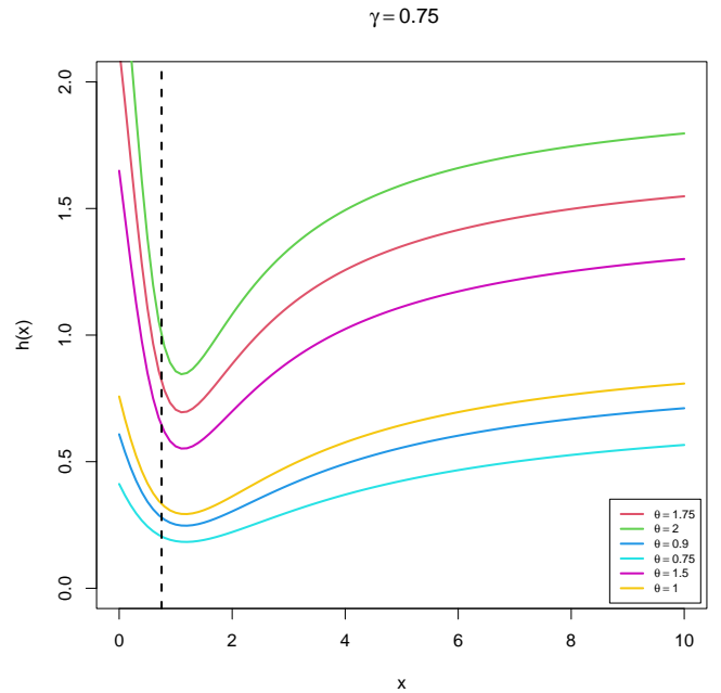
Figure 4: hazard function of the SHCJ dist.
