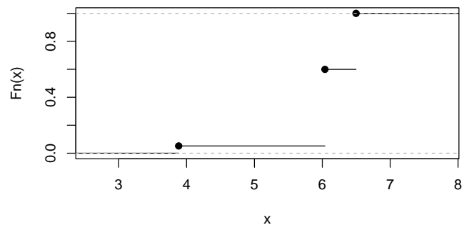
Figure 8: Cumulative function plot for \theta
