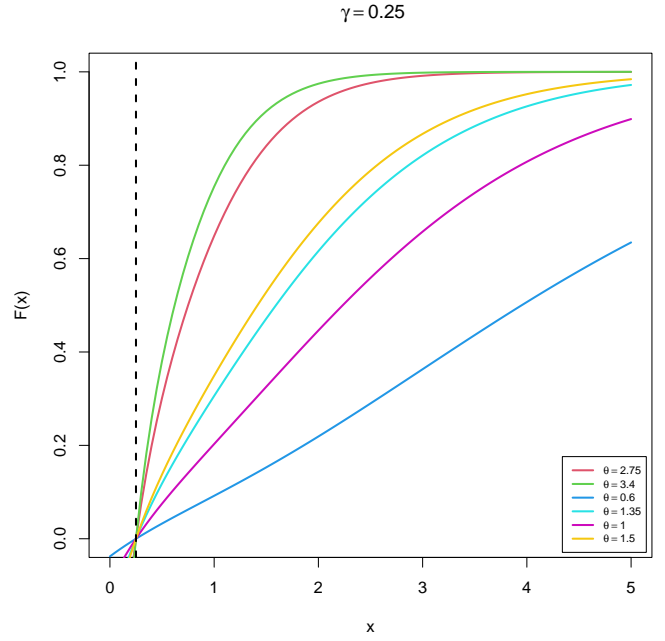
Figure 2: cdf of the Shifted Chris-Jerry Dist.
