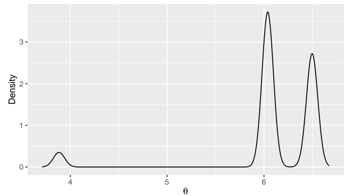
Figure 10: Marginal Posterior function plot for \theta
