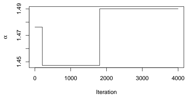
Figure 11: Trace plot for \alpha
