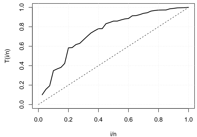
Figure 16: TTT Plot
