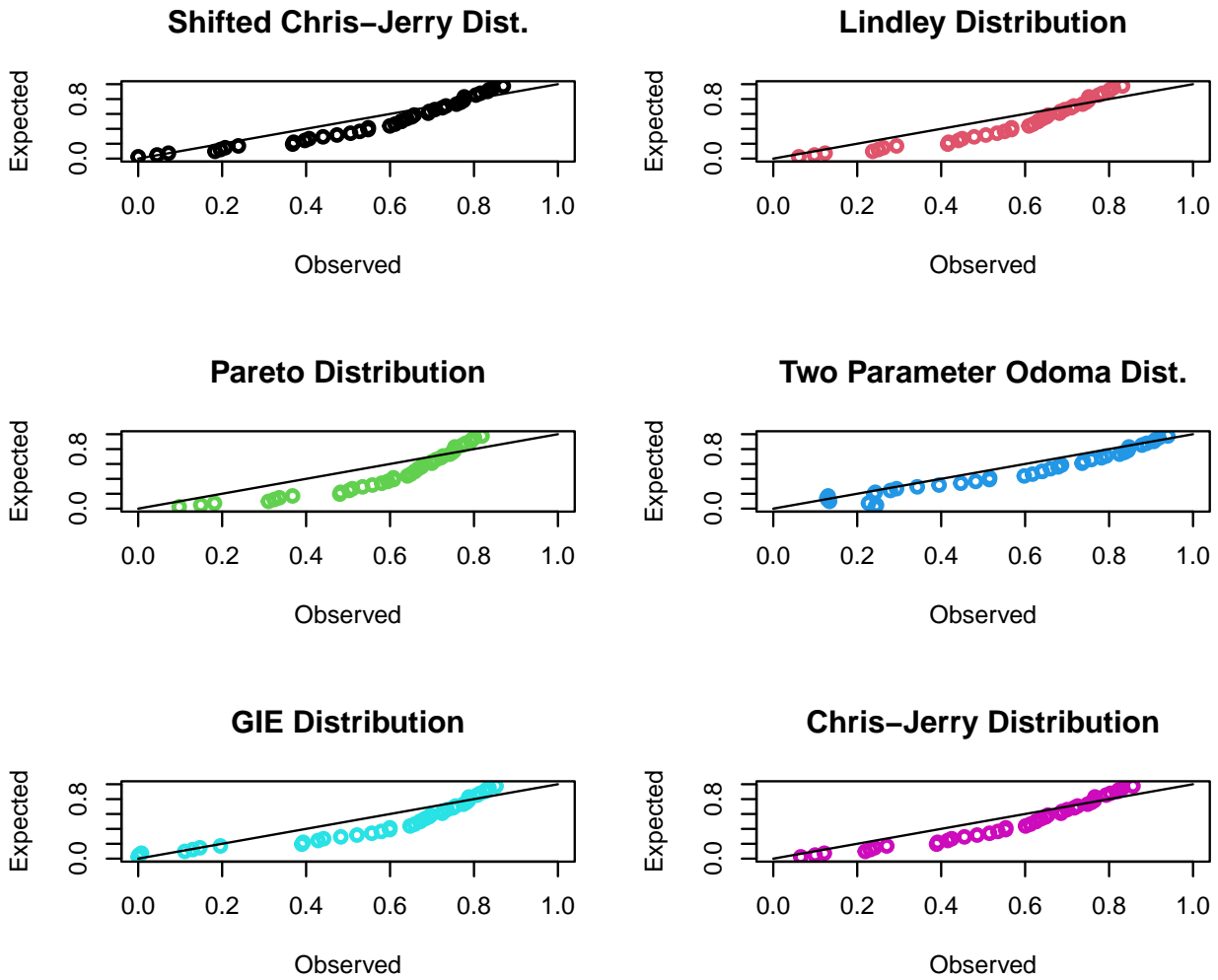
Figure 17: PP plots
