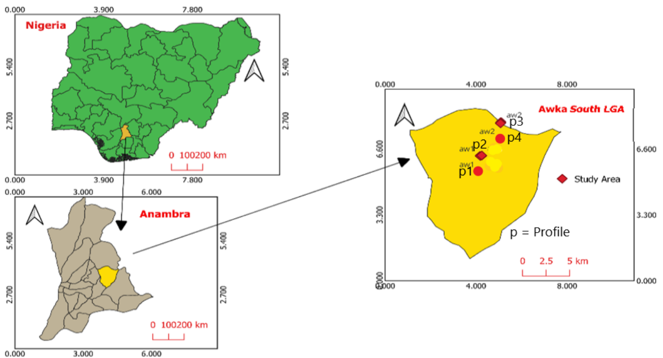
Figure 1. Map of the geological setting of Nigeria and Anambra Basin, [39]
