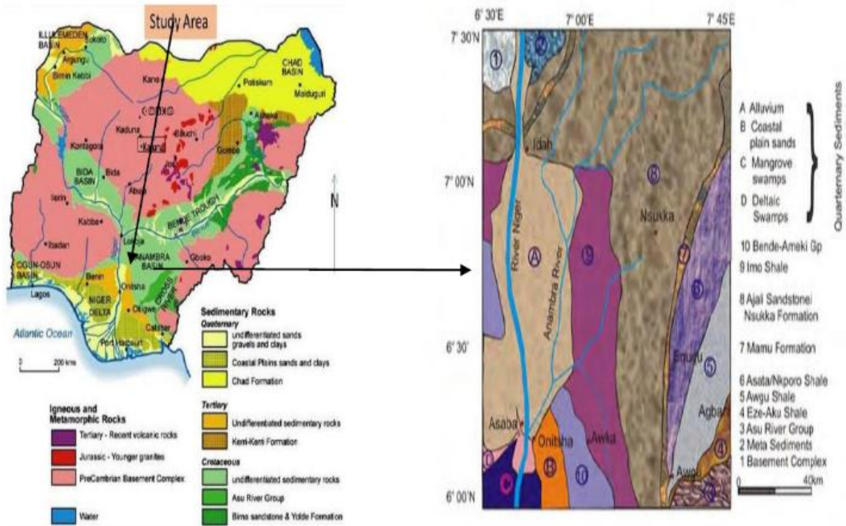
Figure 1. Map of the geological setting of Nigeria and Anambra Basin, [39]
