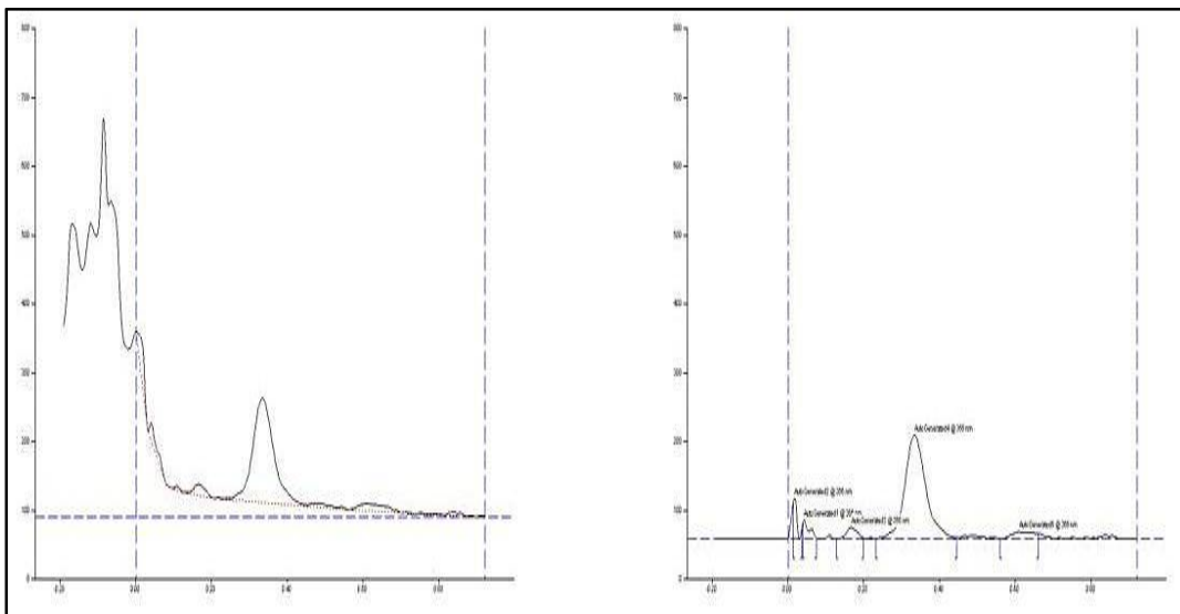
Fig 3 HPTLC Fingerprinting of Sample AM
