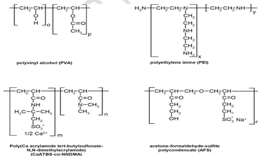
Fig. 1: Chemical Structures of Some Fluid loss Additives
