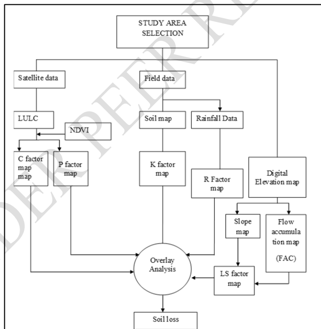
Fig. 2. Flow chart for estimation of soil erosion
